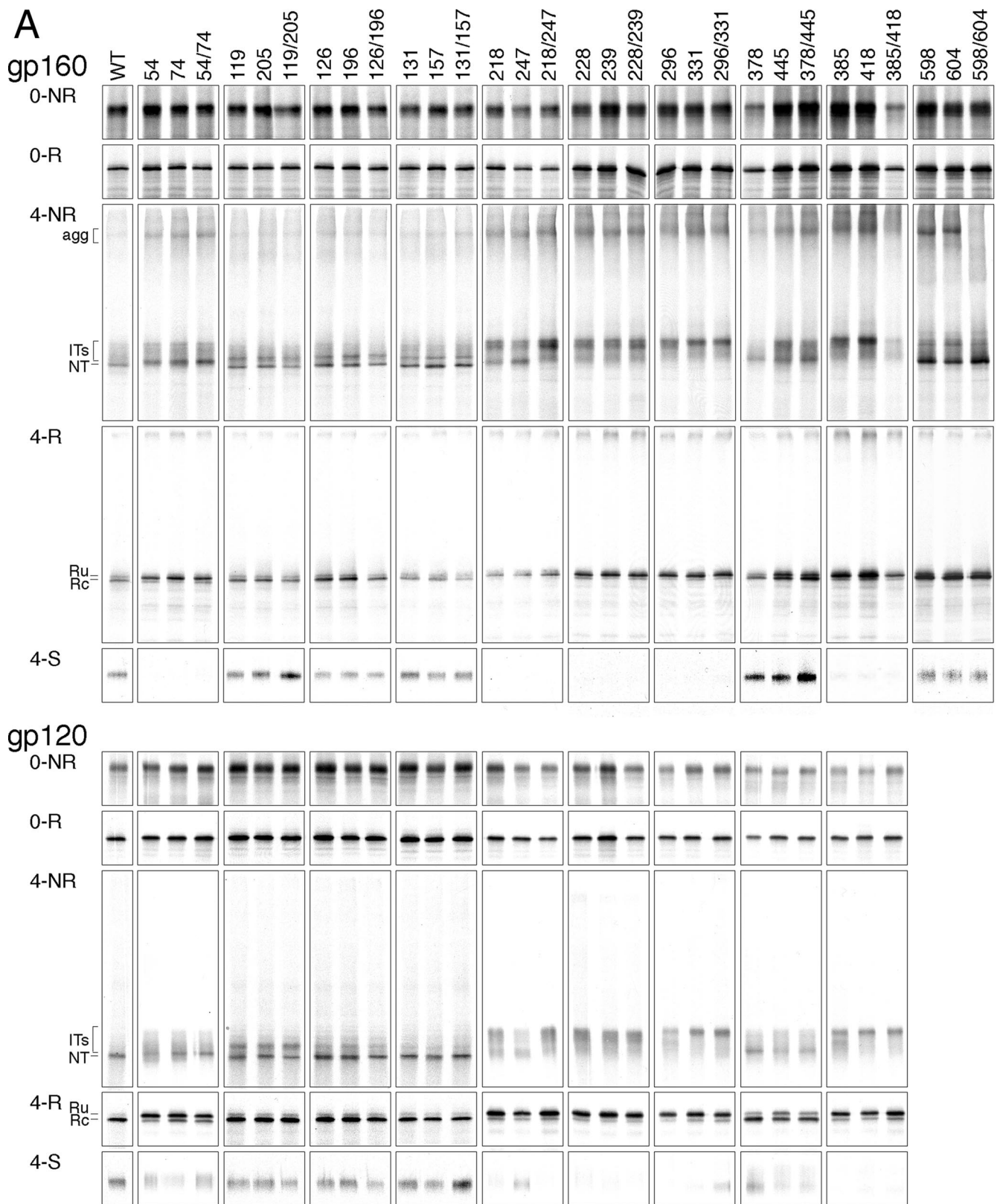
Figure 3. Folding “endpoint” analysis of Env cysteine mutants. (A) Wild-type or cysteine mutants of gp160 or gp120 were expressed in HeLa cells using the Vaccinia T7 heterologous expression system. Cells were pulse-labeled for 10 min and chased for 0 or 4 h. Cells were lysed and Env proteins were immunoprecipitated from lysates and chase medium. Samples were analyzed as in Figure 2. (B) Data were quantified with ImageQuant (Molecular Dynamics, Sunnyvale, CA), and percentage aggregation, NT formation, Rc formation, and shedding/secretion are depicted in histograms.
