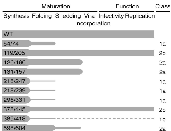
Figure 7. Classification of disulfide bonds of Env. HIV-1 Envelope disulfide mutants were clustered in four classes based on the “bottlenecks” in their maturation and/or function in comparison to wild-type. Bottlenecks are depicted on an arbitrary scale. Class 1a mutants are incompetent for folding and function; class 1b mutants display residual viral function (depicted by a dashed line) despite severe folding problems; class 2a mutants are folding competent, but function incompetent. Finally, class 2b mutants are folding and function competent. For clarity, only double mutants are shown in this cartoon.
