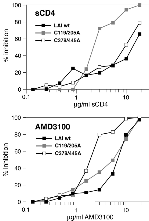
Figure 6. Effect of inhibition of (co-)receptor binding on replicating mutant viruses. CD4^+ lymphocytes ( 2.0 \times 10^5 /well in 96-well plates) were inoculated with equal amounts (100 TCID 50 ) of the parental HIV-1 LAI or mutant virus containing Env lacking either the 119–205 or the 378–445 disulfide bond. CD4 receptor binding was inhibited by limiting dilutions of sCD4 (top) and CXCR4 coreceptor binding with AMD3100 (bottom). As a measure for inhibition, the percentage reduction in CA-p24 production at various concentrations of either compound as compared with the CA-p24 production in the absence of compound was calculated. The experiment was repeated several times, and results were reproducible.
