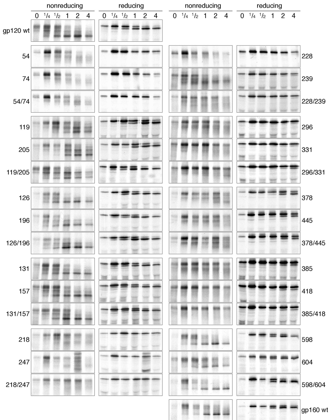
Figure 4. Folding kinetics of Env cysteine mutants. Wild-type or cysteine mutants of gp120 as well as 598–604 disulfide mutants of gp160 were expressed in HeLa cells using the Vaccinia T7 heterologous expression system. Cells were pulse-labeled for 2 min (gp120) or 5 min (gp160) and chased for various times (h) as indicated. Cells were lysed and Env proteins were immunoprecipitated from lysates, deglycosylated with endoH, and analyzed by nonreducing (NR) or reducing (R) 7.5% SDS-PAGE.
