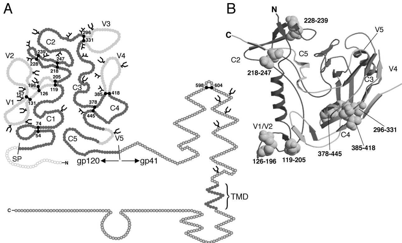
Figure 1. Schematic representation of the gp160 precursor of HIV Envelope. (A) Residues are displayed as spheres. The soluble subunit gp120 with constant (C) – in dark gray – and variable (V) – in light gray – domains and the signal peptide (SP) – in white, and the transmembrane subunit gp41 with its transmembrane domain (TMD) – in darker gray – are indicated. Disulfide bonds (with residue numbers of cysteines) and attached glycans of both the complex ( \cup ) and oligomannose/hybrid type ( \nabla ) as well as the N-terminus (N) and C-terminus (C) are indicated. (B) Ribbon representation of the crystal structure of gp120 (Kwong et al. , 1998). Atoms of cysteine pairs are shown as space filling spheres. Note that the C1 region including the 54–74 disulfide bond is absent. Only the stem of the V1/V2 loops is present, excluding the 131–157 disulfide bond, and the V3 and V4 loops are absent from the core crystal structure of gp120.
