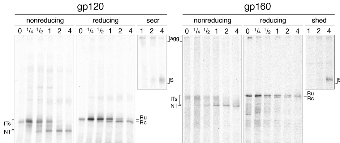
Figure 2. Folding of wild-type gp160 and gp120. Wild-type Env, as precursor gp160 or as the soluble subunit gp120 alone, was expressed in HeLa cells using the Vaccinia T7 heterologous expression system. Cells were pulse-labeled for 2 min (gp120) or 5 min (gp160) and chased for various times (h) as indicated. Cells were lysed and Env proteins were immunoprecipitated from lysates and from the chase medium. Immunoprecipitates from lysates were fully deglycosylated with endoH (see Materials and Methods ) and analyzed by nonreducing (NR) or reducing (R) 7.5% SDS-PAGE. Immunoprecipitates from the chase media of secreted or shed (S) gp120 were analyzed directly on reducing 7.5% SDS-PAGE. Aggregates (agg), folding intermediates (ITs), the native form (NT), and the reduced protein from which the signal peptide was cleaved off (Rc) or not (Ru), as well as the shed or secreted gp120 (S) are indicated.
