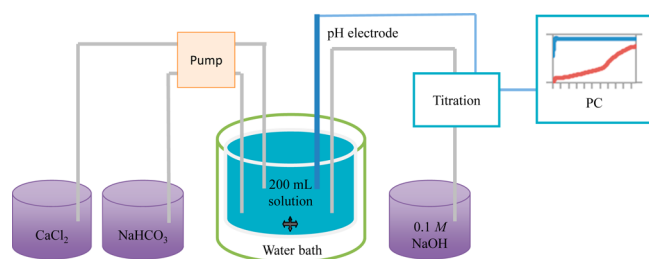
Figure 1. Experimental setup for calcium carbonate precipitation under varied experimental conditions at near-freezing temperature.
