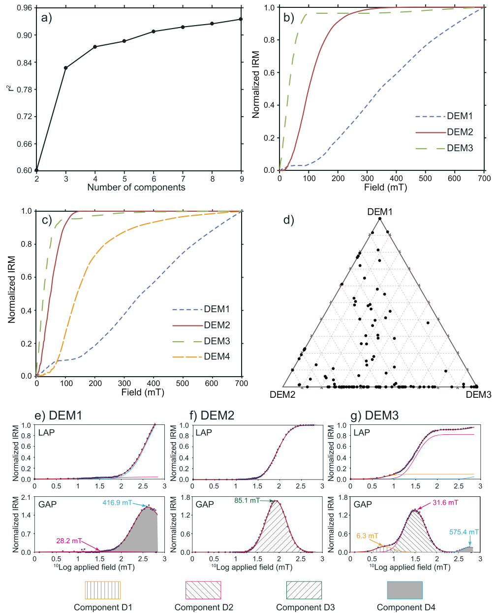
Figure 8. End-member modeling for volcanic rocks from E_{1d} . (a) Diagram showing the r^2 versus number of end members. (b and c) End members for the normalized IRM acquisition curves in the (b) three and (c) four end-member models. (d) Ternary plot of the three end-member model showing the end-member percentages for individual specimens. (e–g) IRM component analysis [Kruiver et al. , 2001] of the end members in the preferred three end-member model. Squares are the calculated data points from end-member modeling that are used to fit the IRM components. The components are marked with different lines: the linear acquisition plot (LAP) and the gradient acquisition plot (GAP) are shown. Component D1 has a very low coercivity and contribution; it is not assigned a physical meaning. Components D2 and D3 are harder; they represent Ti-poor and Ti-rich titanomagnetite, respectively. Component D4 has the highest coercivity and shows properties characteristic of hematite. IRM is normalized to the highest IRM value ( IRM/IRM_{700 \text{ mT}} ); \log_{10}(B_{1/2}) and DP are in \log_{10} mT. Values of B_{1/2} are displayed on each panel.
