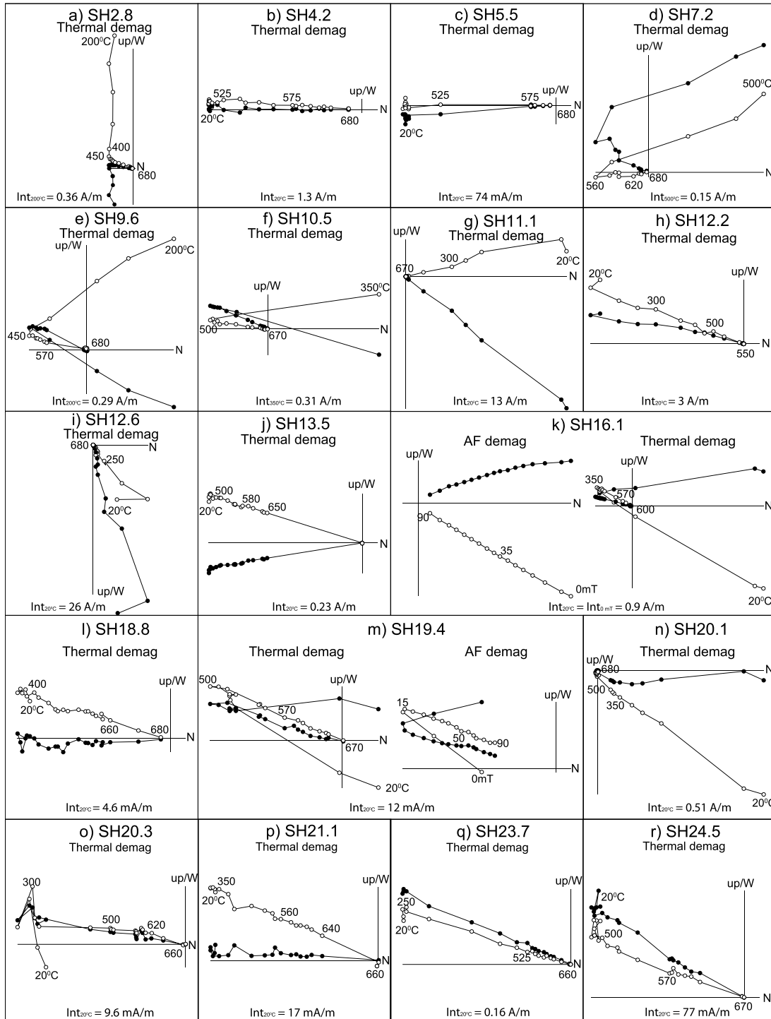
Figure 4. Demagnetization diagrams for samples representing the entire E_{1d} interval. All diagrams are displayed after bedding tilt correction. Closed (open) symbols represent the projection of vector end-points on the horizontal (vertical) plane; values represent alternating field and thermal demagnetization steps in milliTesla (mT) and °C, respectively. Most of the samples only yielded interpretable results when processed with thermal demagnetization (a–j and i–r); AF demagnetization can only remove part of the low-temperature component (e.g., SH16.1 in k). Few samples (SH19.4, m) yield comparable characteristic remanent magnetizations by AF and thermal treatments.
