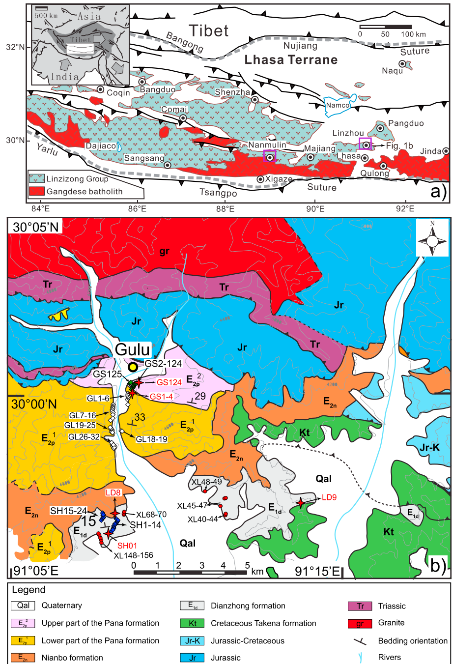
Figure 1. (a) Simplified geological map showing the distribution of the Gangdese batholith and associated Linzong volcanic successions in the Lhasa terrane, southern Tibet [modified from Yin and Harrison, 2000; Lee et al. 2009]; (b) simplified geologic map of the Linzhou basin [modified from He et al., 2007]. Diamonds and dots represent paleomagnetic sampling locations: white diamond—Dupont-Nivet et al. [2010b] from lower E 2p , green diamond—Huang et al. [2013] from upper E 2p , and blue diamond—this research from E 1d . Red dot: Chen et al. [2010] and Chen et al. [2014] from E 1d . Red stars represent geochronological sampling locations.
