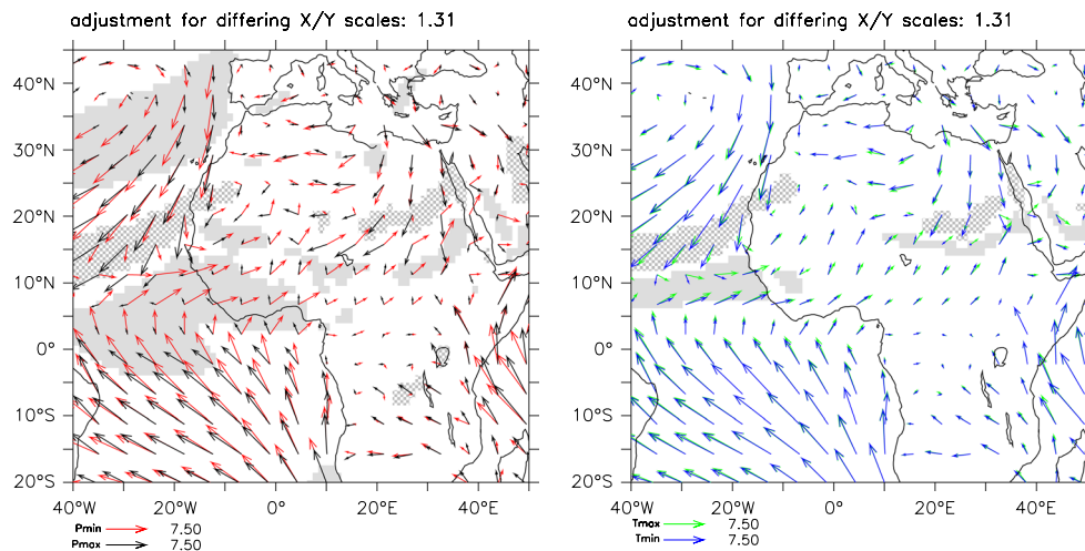
Fig. 8 June–July–August average surface winds in m/s in the Pmin experiment (left, red), Pmax (left, black), Tmax (right, green), Tmin (right, blue). Differences in wind speed are given by grey shading;
