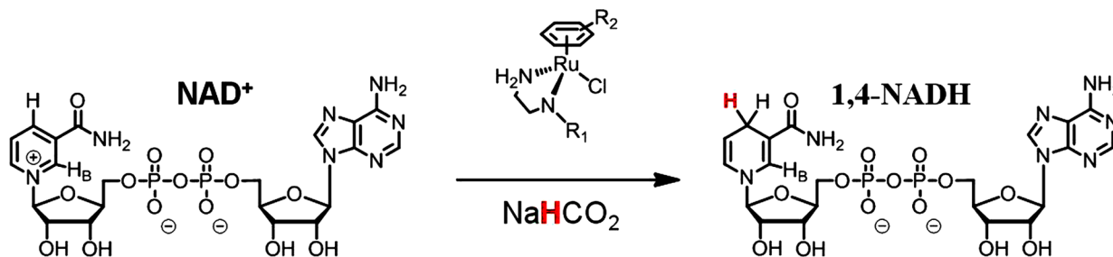
Scheme 1. Reduction of NAD + to 1,4-NADH in the Presence of Formate as a Hydride Source
