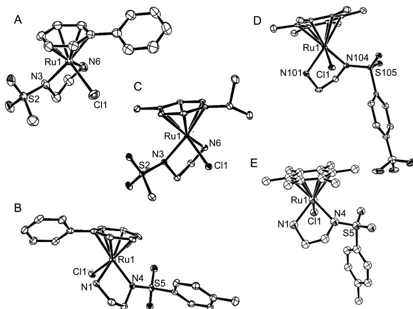
Figure 1. ORTEP diagrams for complexes (A) 7, (B) 8, (C) 1, (D) 6, and (E) 5. Ellipsoids are shown at the 50% probability level. All hydrogen atoms and solvent molecules have been omitted for clarity.
