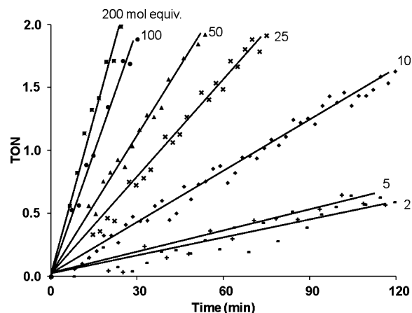
Figure 2. Dependence of the turnover number on time for the reduction of \text{NAD}^+ by complex 2 using formate as a hydride source (mol ratio 2:1: X , X = 2, 5, 10, 25, 50, 100, \text{ or } 200 . \text{pH}^* 7.4, 310 \text{ K}, \text{D}_2\text{O} ).
