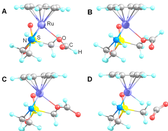
Figure 4. Calculated DFT structures for the formate adduct of {(bn)Ru(MsEn)} + (from 10). (A) Intermediate complex with formate bound via a single oxygen with an H-bond between the second formate oxygen and NH from the chelating ligand. (B) Transition state for the rotation of formate that begins to orient the hydrogen toward the metal center. (C) Intermediate showing the hydrogen now oriented toward the Ru center, and finally (D) the transition state for the formation of the ruthenium-hydride bond and CO 2 elimination. Imaginary frequencies for B and D were 148i and 329i cm -1 , respectively.
