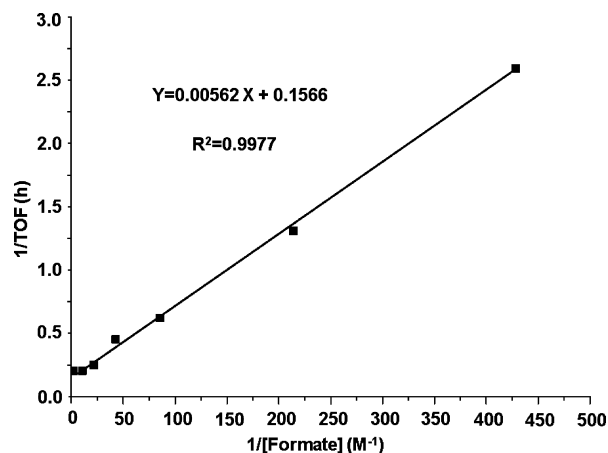
Figure 3. Plot of the reciprocal of the TOF against formate concentration for the reduction of \text{NAD}^+ in the presence of various molar equiv of formate, catalyzed by complex 2 . For a reaction following Michaelis-type kinetics, \text{TOF} = \text{TOF}_{\text{max}}[\text{S}]/(K_m + [\text{S}]) , where \text{TOF}_{\text{max}} is the turnover frequency at infinite substrate (formate) concentration, [\text{S}] is the substrate concentration, and K_m is the Michaelis constant. Hence, \text{TOF}^{-1} = (K_m/\text{TOF}_{\text{max}})(1/[\text{S}]) + (1/\text{TOF}_{\text{max}}) , and K_m and \text{TOF}_{\text{max}} can be obtained from the gradient and y intercept, respectively, of the double-reciprocal plot.
