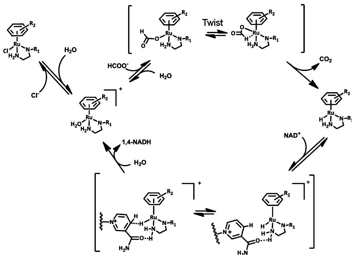
Scheme 2. Proposed Mechanism for Reduction of NAD + to 1,4-NADH via Transfer Hydrogenation Using Formate as the Hydride Source a
