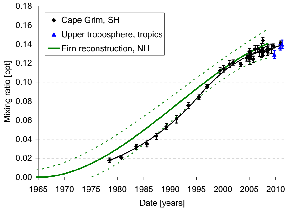
Fig. 2. Same as in Fig. 1 but for n\text{-C}_5\text{F}_{12} .
