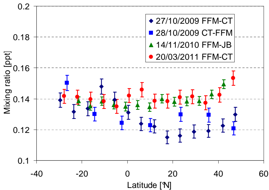
Fig. 6. Same as in Fig. 5 but for n\text{-C}_5\text{F}_{12} .
