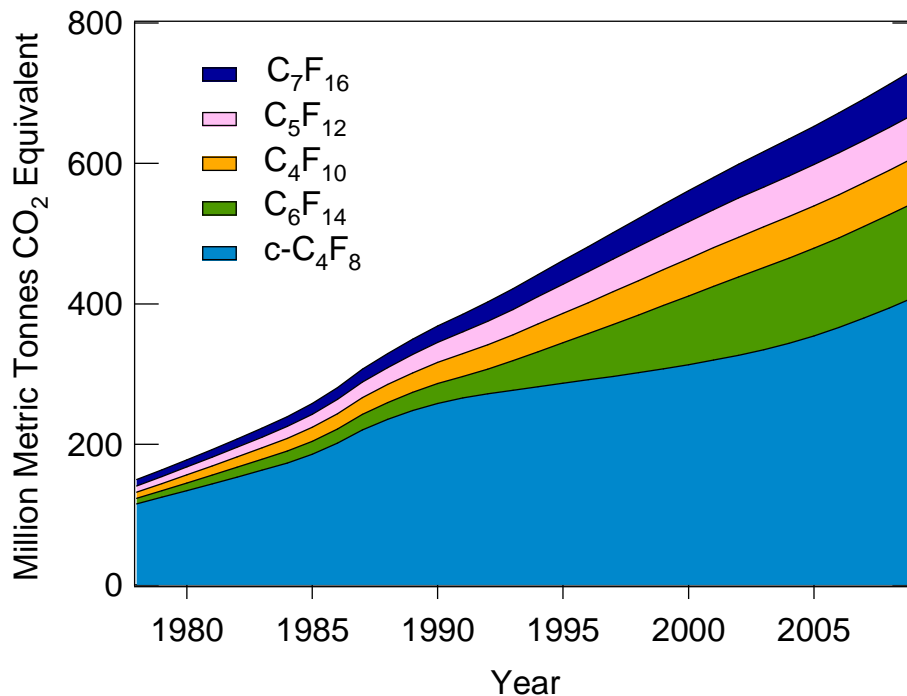
Fig. 10. Cumulative emissions of C 4 to C 7 perfluorocarbons: the four compounds reported here plus those of c -C 4 F 8 as updated from Oram et al., 2012 in mt (million metric tonnes) of CO 2 equivalent. The Global Warming Potentials (GWPs) reported in IPCC, 2007 were applied to derive these emissions. As no GWP is reported for n -C 7 F 16 in IPCC, 2007 and Bravo et al., 2010 we assumed a similar GWP to that of n -C 6 F 14 .
