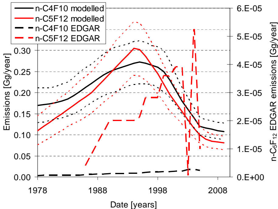
Fig. 8. Time series of the global emissions of n\text{-C}_4\text{F}_{10} (black) and n\text{-C}_5\text{F}_{12} (red) modelled from the Cape Grim trends (solid lines) in gigagrams (Gg) per year as compared to emissions reported by the EDGAR emission database (long-dashed lines, EDGAR, 2010). Please note that the EDGAR emissions for n\text{-C}_5\text{F}_{12} are very small and thus plotted on a separate y-axis. The short-dashed lines are uncertainty estimates consisting of a) the 1\sigma measurement standard deviations plus b) the square root of the sum of the squares of the of the deviation of the actual mixing ratios from the polynomials fitted to derive the growth rates plus c) an additional calibration scale uncertainty (see Supplement).
