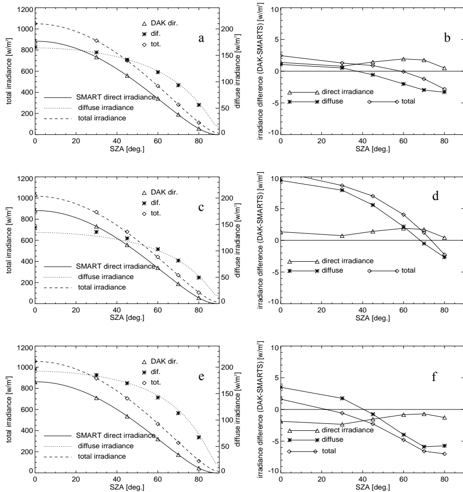
FIGURE 3. Similar as Fig. 2 but with LOWTRAN aerosols, AOT=0.2 at 500 nm. (a, b) rural aerosol, (c,d) urban aerosol, (e,f) maritime aerosol.
