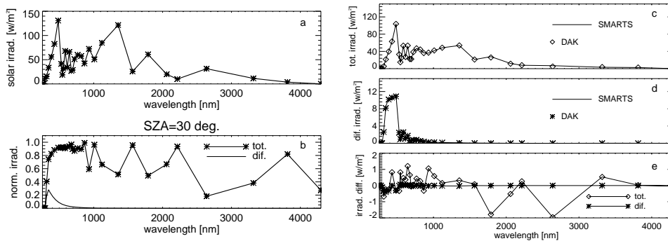
FIGURE 1. Left: (a) Solar spectrum at TOA at 32 wavelength bands. (b) DAK simulated total and diffuse irradiance spectra. The spectra are normalized. Right: DAK and SMARTS simulated (c) total irradiance spectra, (d) diffuse irradiance spectra, and (e) the differences. All the simulated spectra are at SZA = 30^\circ .
