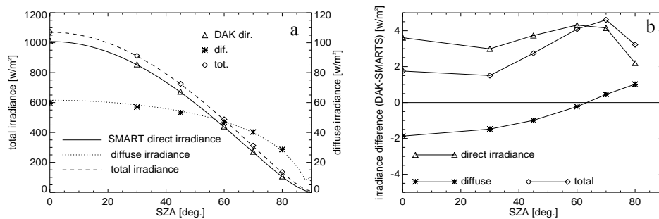
FIGURE 2. (a) DAK and SMARTS simulated direct, diffuse and total irradiances for a pure Rayleigh atmosphere. (b) The differences (DAK-SMARTS).
