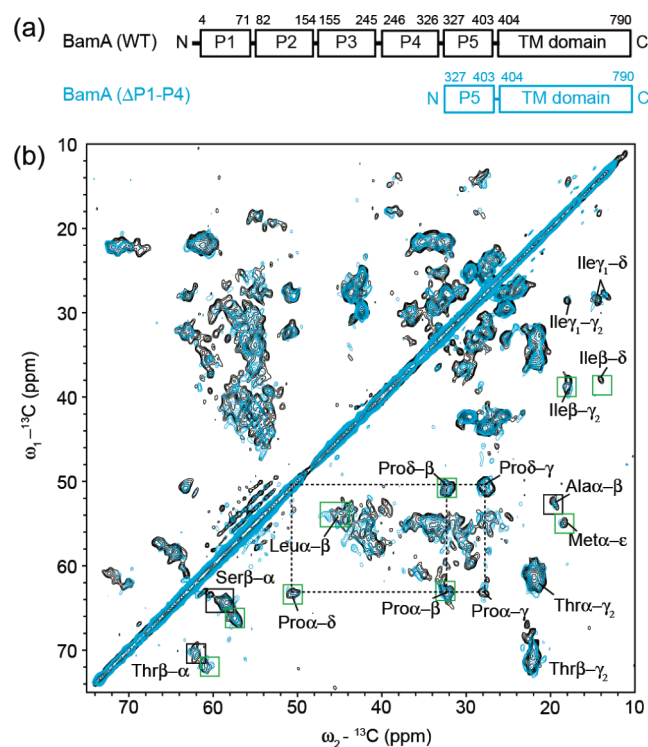
Figure 1. (a) Domain organization within the full-length BamA protein (WT) and the BamA( \Delta P1–P4) variant. (b) Overlay of the aliphatic region of the 2D ^{13}\text{C} – ^{13}\text{C} PDSB spectra (mixing time 40 ms) recorded on BamA precipitate (black) and reconstituted BamA( \Delta P1–P4) variant (blue) with 10.92 kHz magic-angle spinning (MAS) and an ^1\text{H} Larmor frequency of 700 MHz. Amino acid-specific assignments are indicated. Characteristic \beta -sheet-like or putative loop CC correlations are shown in green and black squares, respectively. See the SI for close-ups of these spectra.
