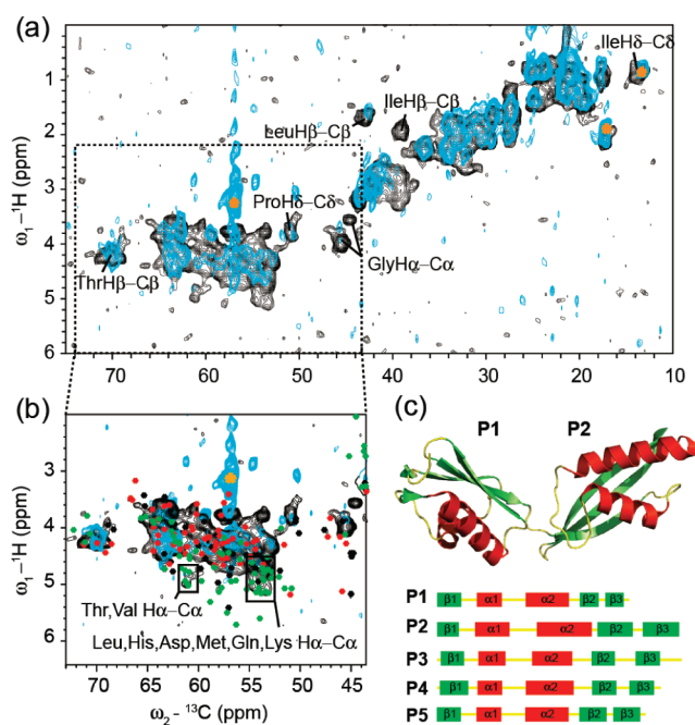
Figure 2. Flexible BamA POTRA domains revealed by scalar-based HC correlation experiments. (a) Overlay of 2D ^1\text{H} – ^{13}\text{C} INEPT spectra (optimized ^1\text{J}_{\text{HC}} = 155 Hz) recorded on BamA precipitate (black) and reconstituted BamA( \Delta P1–P4) variant (blue) with 10.92 kHz MAS and an ^1\text{H} Larmor frequency of 700 MHz. Amino acid-specific assignments are indicated. (b) Selected region of the 2D ^1\text{H} – ^{13}\text{C} INEPT spectra showing backbone HC correlations of BamA proteins. Characteristic \beta -sheet-like \text{H}\alpha – \text{C}\alpha correlations are shown in squares. Lipid resonances are indicated with orange stars. Available solution NMR chemical shifts of the POTRA1 and POTRA2 domains (BMRB entry 15247; see ref 9) are indicated with colored circles ( \alpha -helix in red, \beta -sheet in green, and random coil in black). (c) Top panel: Cartoon representation of the solution NMR structure of isolated BamA POTRA domains P1–P2 (PDB entry 2V9H; see ref 9) used for ssNMR data analysis. Bottom panel: distribution of secondary structure elements present within the POTRA domains of BamA, as seen in the available high-resolution 3D structures of isolated BamA POTRA domains (PDB entries 2V9H, 9 2QDF, 6 and 3OG5 16 ). See the SI for close-ups of these spectra.
