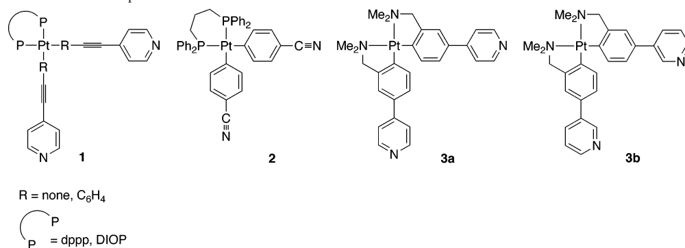
Chart 1. Organometallic Corner Complexes
