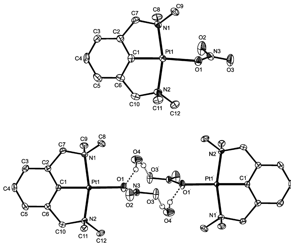
Figure 2. Displacement ellipsoid plot (50% probability level) of the molecular structure of 11a (top) and a dimeric 11a·H 2 O (bottom), with the adopted labeling schemes. Hydrogen atoms (except for the water molecule) have been omitted for clarity (symmetry operation i : 1 - x , 1 - y , 1 - z ). Note that the H 2 O molecules represent the bridges between the neutral [Pt(NCN)(NO 3 )] entities.
