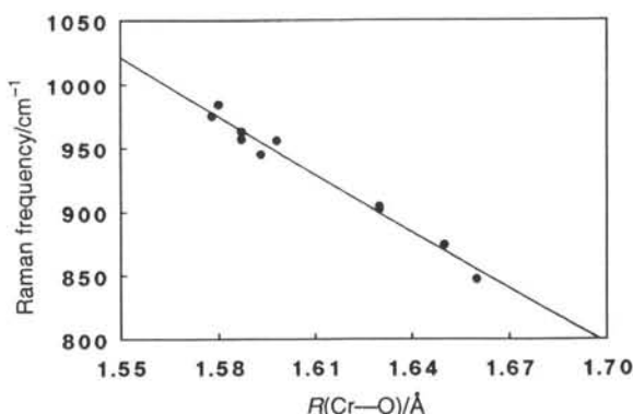
Fig. 1 Correlation plot relating Cr—O bond lengths ( \text{\AA} ) to Cr—O stretching frequencies ( \text{cm}^{-1} ). The data points are fit to an exponential function [eqn. (4)].
