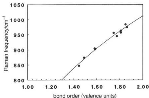
Fig. 2 Correlation plot relating Cr—O bond strength (in valence units) to Cr—O stretching frequencies ( \text{cm}^{-1} ), according to eqn. (5).
