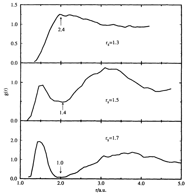
FIG. 2. Pair correlation functions with "cold" electrons ( T = 1000 K).
