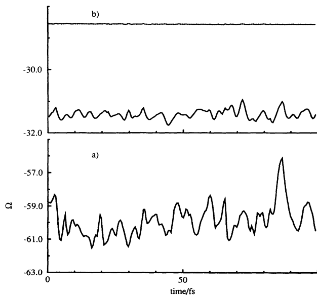
FIG. 1. Example of energy conservation during a microcanonical run. (a) \Omega , (b) solid line: \mathcal{F} , dotted line: \mathcal{F} + K , where K is the ionic kinetic energy. All energies are in atomic units.
