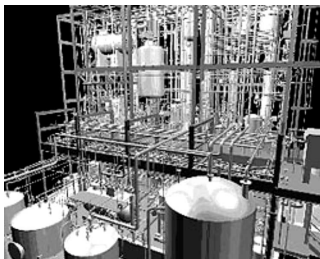
Figure 5.1: CAD model of a carbon black unit. Designed by OLAJTERV Process and Energy, Hungary.
