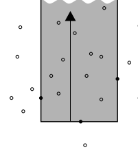
Figure 2.5: The extreme point for the first direction of the sequence, +x_2 , must be the (\tau n) 'th point in the shaded area.
