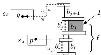
Figure 7.9: Proof of Lemma 7.4.4.
