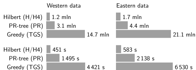
Figure 4.11: Bulk-loading performance on TIGER data: I/O (upper figure) and time (lower figure).
