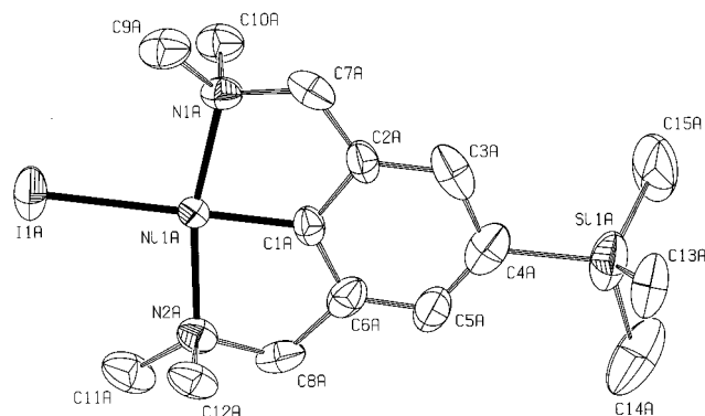
Figure 2. Displacement ellipsoid plot (ORTEP, 50% probability) of one of the two crystallographically independent molecules of [\text{NiI}(\text{C}_6\text{H}_2\{\text{CH}_2\text{NMe}_2\}_2\text{-2,6-SiMe}_3\text{-4})] ( 5 ) in the solid state together with the adopted numbering scheme. For a complete figure, see Supporting Information. Hydrogen atoms have been omitted for clarity.
