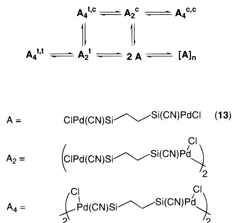
Figure 4. Possible aggregation modes and isomeric forms for the (\text{CN})\text{PdCl} -dimeric units in the dipalladium carbosilane compound 13 .
