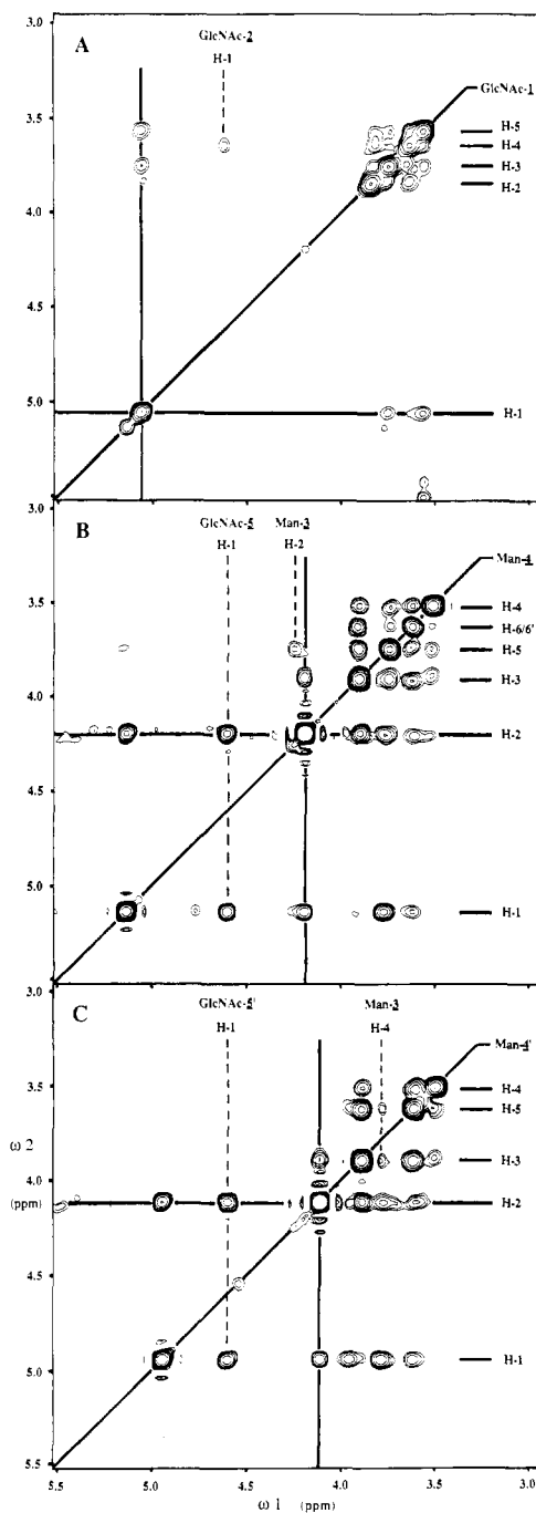
Figure 2. Cross sections perpendicular to the \omega_3 axis of the 3D NOE-HOHAHA ^1\text{H} spectrum of a 20 mM solution of 1 in \text{D}_2\text{O} at 304 K and \text{pH} = 7 . Cross sections are shown at the \omega_3 resonance positions of GlcNAc-1 H-1 (A), Man-4 H-2 (B), and Man-4' H-2 (C). The NOE, HOHAHA, and back-transfer lines are indicated. The phase-sensitive spectrum was recorded at 500 MHz on a Bruker AM500 spectrometer by using a phase cycle of four steps on the pulse after the NOE mixing period. Combined with a phase cycle of two steps for axial peak suppression this yielded 8 scans for each FID. Acquisition was preceded by two dummy scans. Positive and negative frequencies in \omega_1 and \omega_2 were separated by independent TPPI on the preparation pulse and the pulse prior to the t_2 evolution period. FIDs were recorded at a size of 1 K. This was repeated independently for 144 incremental t_1 and t_2 values, resulting in a total measuring time of approximately 63 h. During the relaxation delay of 0.45 s the HDO resonance was suppressed by radiation. Spectral width in all three time domains was 2272.7 Hz. The NOE mixing time was 0.35 s. Isotropic mixing was induced by an MLEV-17 sequence of 94 ms with trim pulses at the beginning and the end. Data were zero-filled twice in the t_1 and t_2 domain before Fourier transformation. Cosine bell windows were used in all three time domains. The resulting data set of 256 \times 256 \times 512 points was base line corrected in all frequency domains by a third-order polynomial fit.
