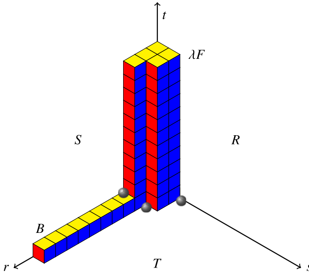
Figure 2. Monomials in the local ring \widehat{\mathcal{O}}_{X,x} \cong \mathbb{C}[[r, s, t]] are represented by cubes. Cubes shown are the monomials in \widehat{\mathcal{O}}_{C,x} . The gray balls are located at monomials which generate \widehat{I}_{C,x} .
