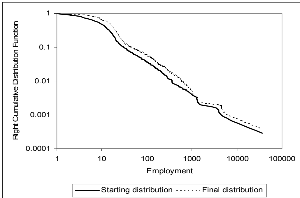
Figure 4a: Cumulative distribution function
