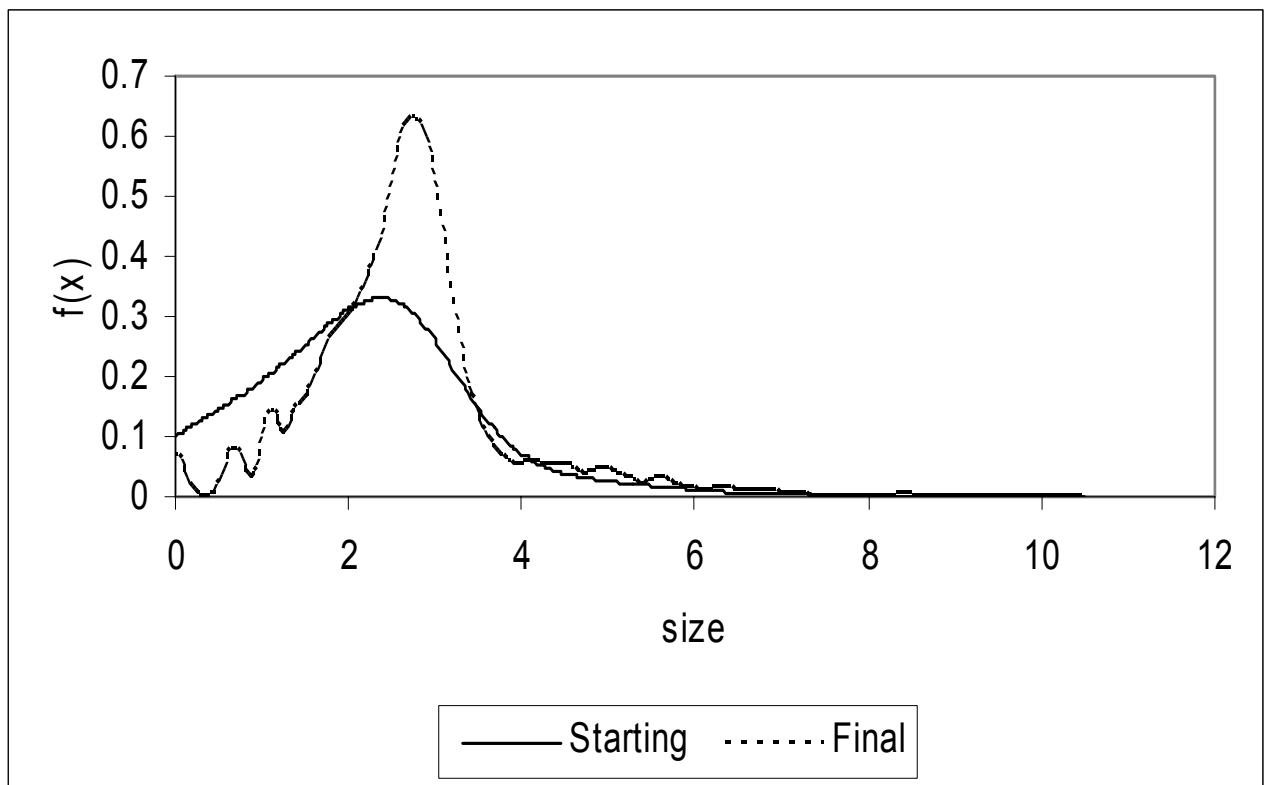
Figure 4b: Probability density function
