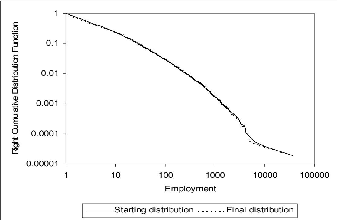
Figure 2a: Cumulative distribution function
