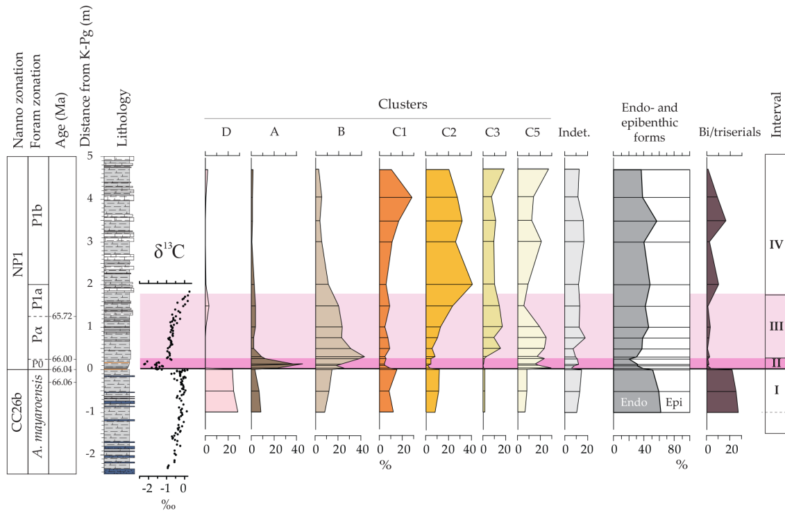
Figure 6. Relative abundances of the four main clusters of benthic foraminiferal taxa (> 125 μm), relative abundances of epibenthic and endobenthic forms, and relative abundance of bi-/triseriate benthic taxa.
