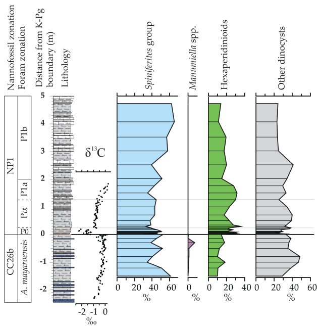
Figure 3. The organic-walled dinoflagellate cyst record of the Okçular section. The biostratigraphy and bulk carbonate stable carbon isotope records are from Açikalin et al. (2015). The four main dinocyst complexes are indicated.
