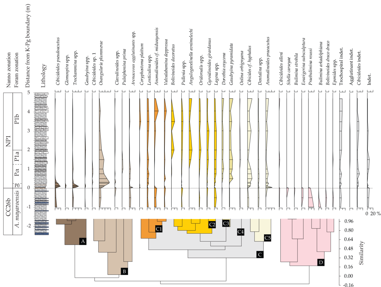
Figure 2. The benthic foraminiferal record (> 125 \mu\text{m} ) of the Okçular section. The biostratigraphy is from Açıkalın et al. (2015). The cluster analysis on the benthic foraminiferal data using paired group (UPGMA) correlation distance allows the identification of four main clusters, A–D, of benthic foraminiferal taxa.
