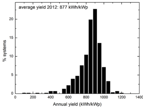
Figure 2. Yield distribution in 2012 in the Netherlands.
