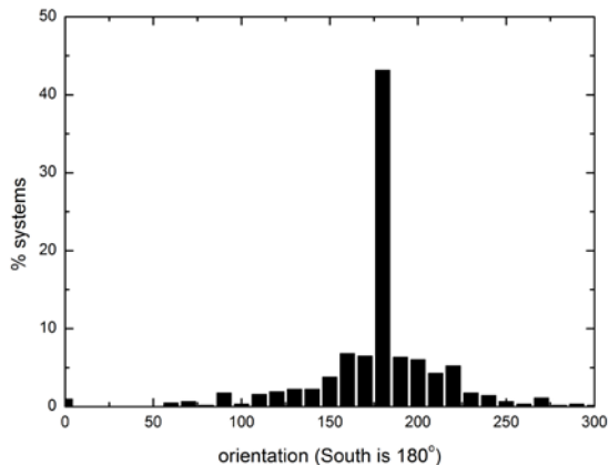
Figure 4. Distribution of orientations.
