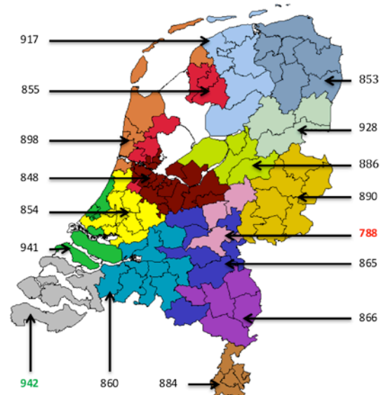
Figure 5. Variation of yield in 2012 in the Netherlands.
