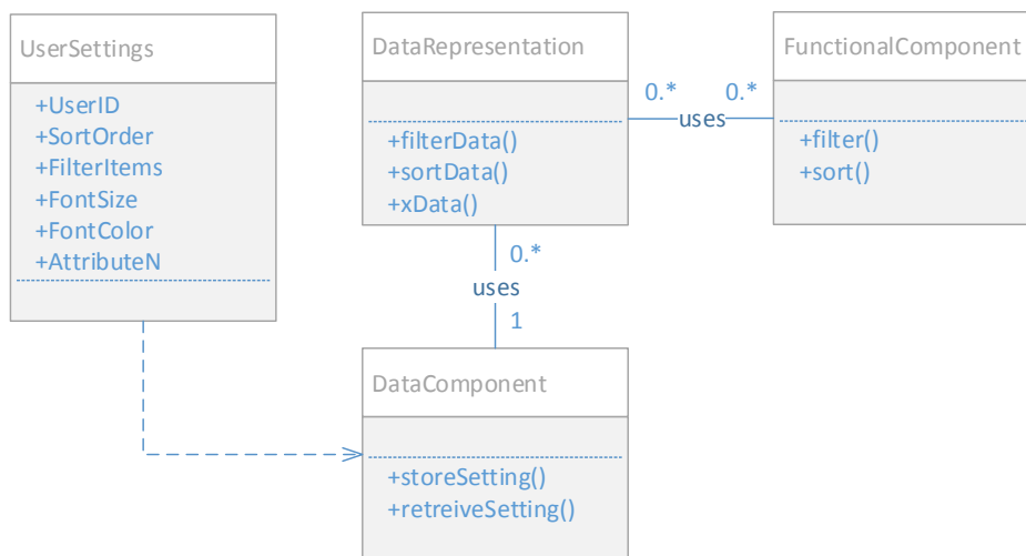
FIGURE A.1: Customizable Data Views Pattern
