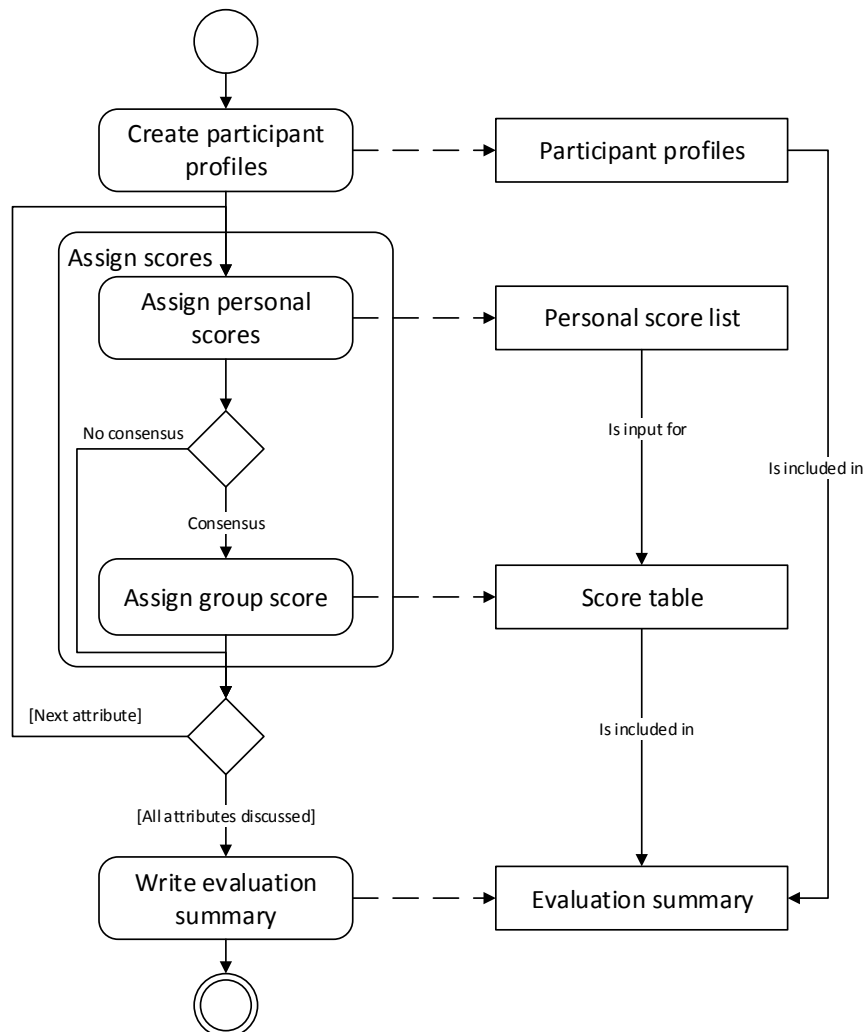
FIGURE 9.4: SPEM: Software Pattern Evaluation Method
