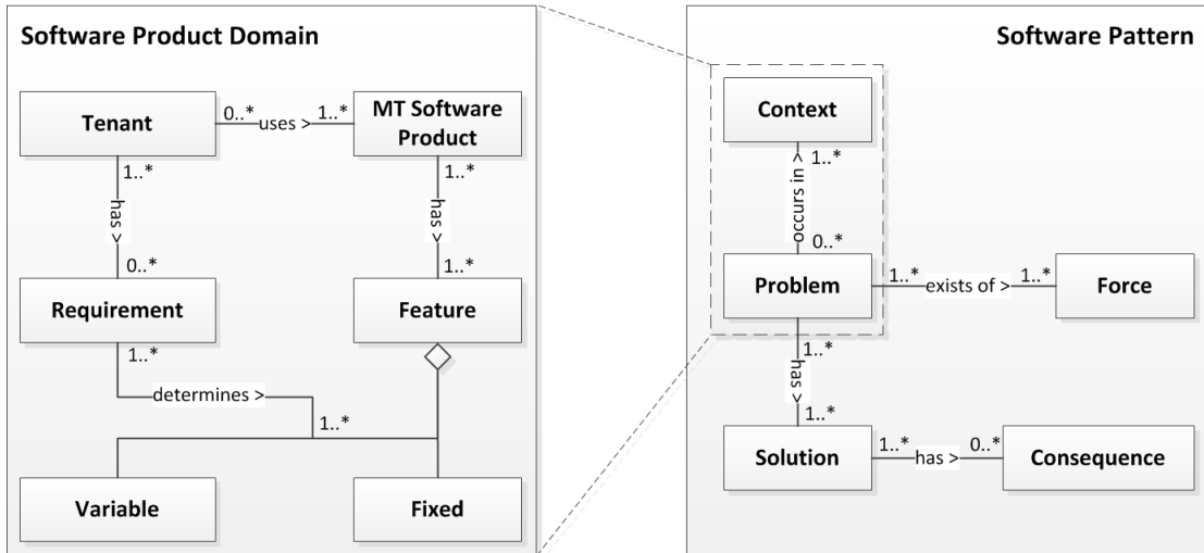
FIGURE 3.1: Conceptual Model: The role of variability patterns in multi-tenant business software
