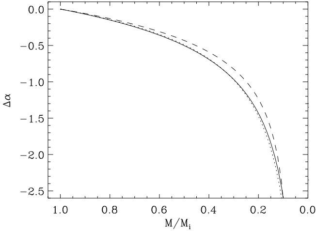
Fig. 3. MF slope change \Delta\alpha in the range m = 0.1\text{--}0.5 M_\odot versus the remaining mass fraction for a Kroupa IMF (solid), Salpeter IMF (dotted), and a power law IMF with \alpha = 1.35 (dashed). In all cases, the IMF mass range is m = 0.1\text{--}1 M_\odot . The displayed relation is valid if stellar evolution is excluded.
