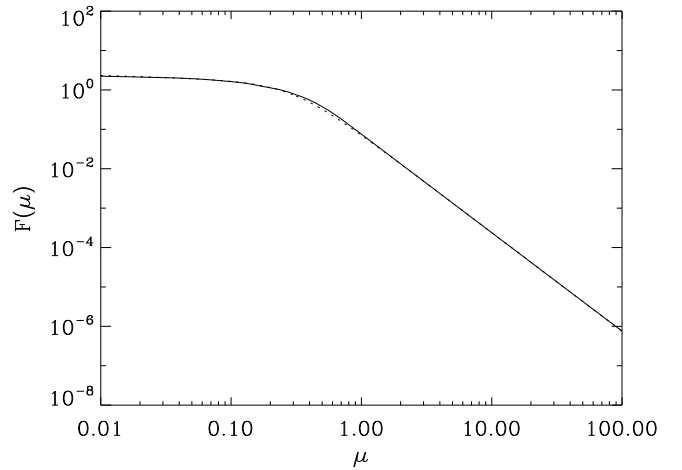
Fig. 2. Hénon function F(\mu) , which is a measure for the escape probability of a star of mass m in a two-body interaction with mass ratio \mu \equiv m/m' . The dotted line shows the fit from Eq. (11).
