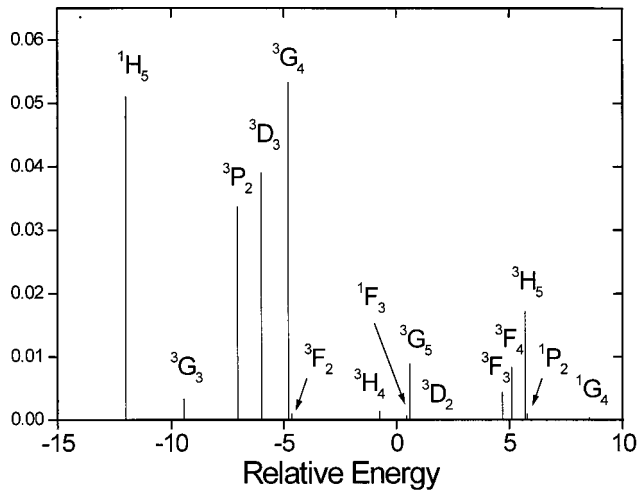
FIG. 2. The theoretical result for the 2p_{1/2}4f^{13} \rightarrow 4d^9 4f^{13} dipole transition. The energy scale is referenced to the average energy of the final state. The relative cross sections are given for the 15 term symbols acquiring finite intensity.
