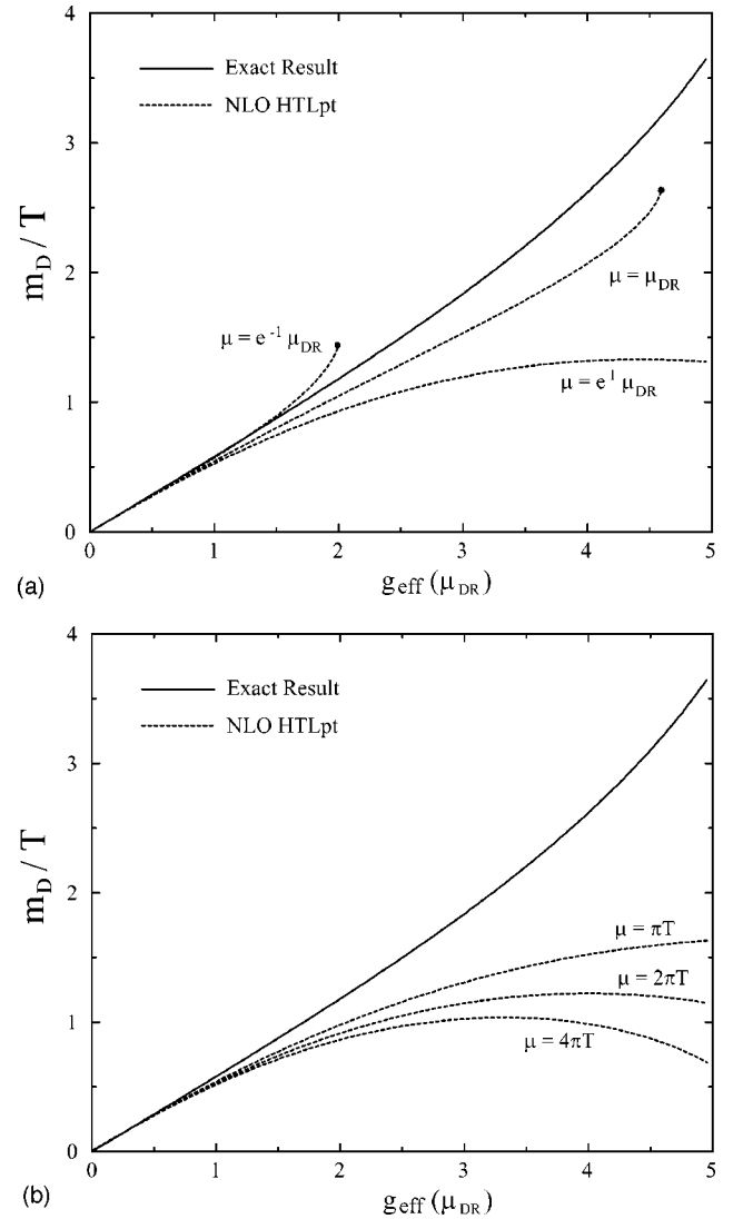
FIG. 7. NLO HTLpt prediction for m_D in the large N_f limit and the exact numerical result [35] as a function of g_{\text{eff}}(\mu_{\text{DR}}) = \sqrt{s_f}g(\mu_{\text{DR}}) = 2\pi\sqrt{s_f}\alpha_s(\mu_{\text{DR}}) where \mu_{\text{DR}} = \pi e^{-\gamma}T . In (a) the renormalization scale \mu is varied by a factor of e around \mu_{\text{DR}} . In (b) the renormalization scale \mu is varied by a factor of 2 around 2\pi T .
