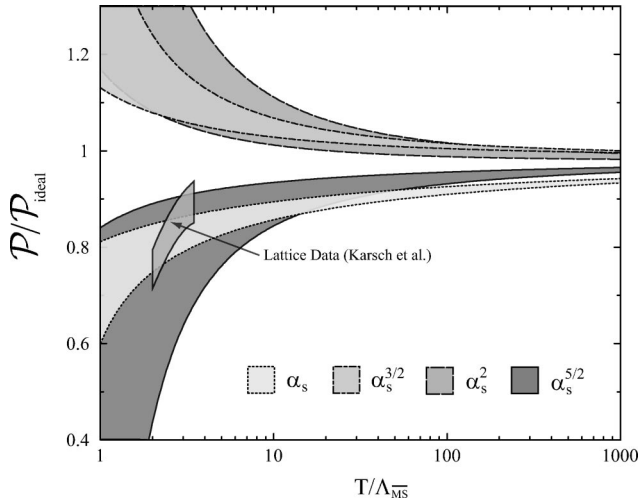
FIG. 1. The perturbative free energy of QCD for N_f=2 massless quarks as a function of T/\Lambda_{\overline{\text{MS}}} . The weak-coupling expansions through orders \alpha_s , \alpha_s^{3/2} , \alpha_s^2 , and \alpha_s^{5/2} are shown as bands that correspond to varying the renormalization scale \mu by a factor of 2 around 2\pi T . Also shown is a lattice estimate by Karsch et al. [7] for the free energy. The band indicates the estimated systematic error of their result which is reported as (15 \pm 5)\% .
