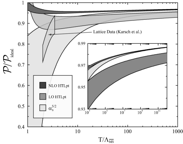
FIG. 4. LO and NLO HTLpt predictions for the free energy of QCD with N_c=3 and N_f=2 together with the perturbative prediction accurate to g^5 . The shaded bands correspond to varying the renormalization scale \mu by a factor of 2 around \mu=2\pi T . Also shown is a lattice estimate by Karsch et al. [7] for the free energy. The band indicates the estimated systematic error of their result which is reported as (15\pm 5)\% .
