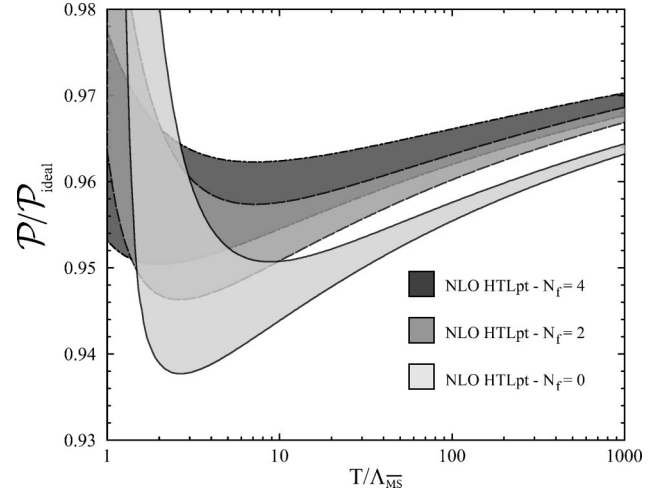
FIG. 5. NLO HTLpt prediction for the free energy of QCD with N_c=3 and N_f=\{0,2,4\} . The shaded bands correspond to varying the renormalization scale \mu by a factor of 2 around \mu=2\pi T .
