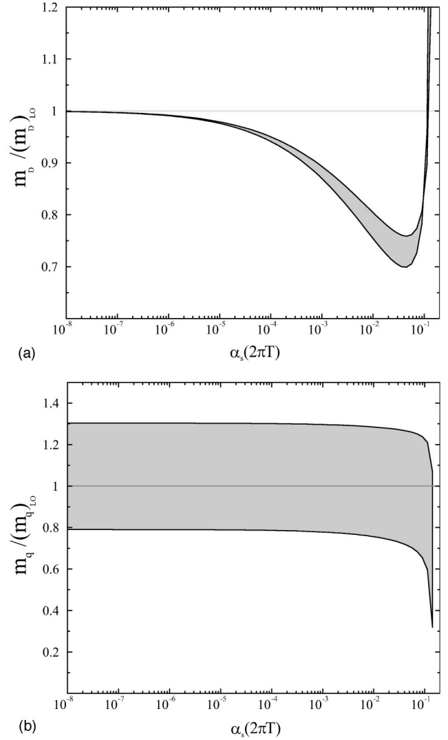
FIG. 3. Numerical solution of gap equations for (a) m_D , Eq. (69), and (b) m_q , Eq. (68), as a function of \alpha_s(2\pi T) for N_c=3 and N_f=3 . The shaded band corresponds to varying the renormalization scale \mu by a factor of 2 around \mu=2\pi T .
