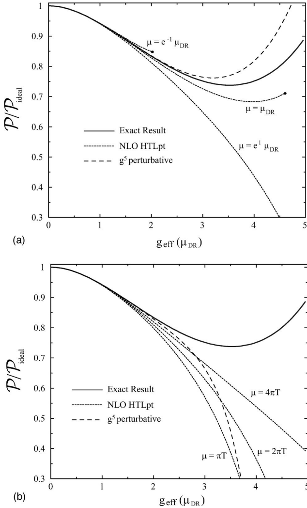
FIG. 6. NLO HTLpt prediction for the O(N_f^0) contribution to the free energy, the numerical result of Ref. [34], and the perturbative prediction accurate to g^5 as a function of g_{\text{eff}}(\mu_{\text{DR}}) = \sqrt{s_f}g(\mu_{\text{DR}}) = 2\pi\sqrt{s_f}\alpha_s(\mu_{\text{DR}}) where \mu_{\text{DR}} = \pi e^{-\gamma}T . Dots indicate the point at which there is no longer a real-valued solution to the gap equation for m_D . In (a) the renormalization scale \mu is varied by a factor of e around \mu_{\text{DR}} . In (b) the renormalization scale \mu is varied by a factor of 2 around 2\pi T . In both (a) and (b) the perturbative g^5 result is evaluated at the central scale.
