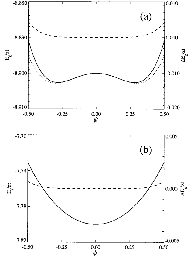
FIG. 3. Ground-state energy (in units of the hopping energy zt ) as a function of \psi for (a) \bar{U}=11 and \bar{\mu}=8.9 and for (b) \bar{U}=11 and \bar{\mu}=7.8 . The solid line represents fourth-order perturbation theory whereas the dotted line represents a numerical diagonalization of the effective hamiltonian. The dashed line is the difference between the two (scale on the right).
