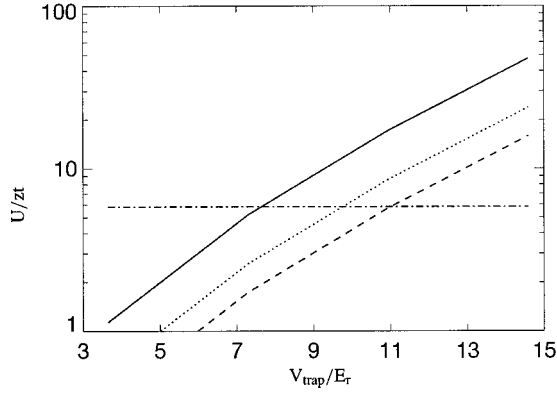
FIG. 9. The dimensionless parameter U/zt plotted as a function of the trap depth (in units of the recoil energy E_r ) for one (solid line), two (dotted line), and three dimensions (dashed line). The dash-dotted line is the critical value \bar{U}=5.83 .
