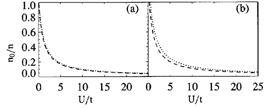
FIG. 1. The condensate fraction n_0/n (a) in a two-dimensional optical lattice and (b) a three-dimensional optical lattice, both as a function of the dimensionless parameter U/t for n=0.5 (dashed line) and n=1.0 (dotted line).
