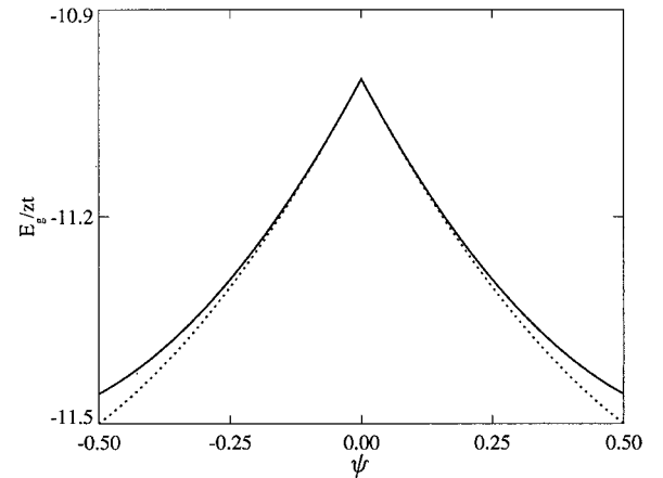
FIG. 4. Ground-state energy (in units of the hopping energy zt ) as a function of \psi for \bar{U} = \bar{\mu} = 11 , as obtained from first-order perturbation theory (solid line) and from numerical diagonalization of the effective hamiltonian (dotted line).
