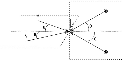
FIG. 7. Laser beam configuration for a three-dimensional optical lattice.
