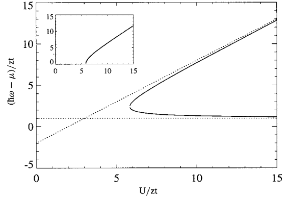
FIG. 6. The quasiparticle and the quasihole energy (in units of the hopping energy zt ) for \mathbf{k}=0 in the g=1 insulator lobe. The dotted lines are the asymptotes of the curves. The inset shows the resulting first-order approximation to the dispersion of the density fluctuations.
