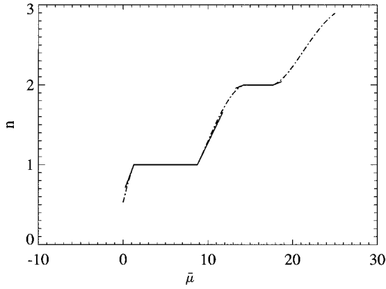
FIG. 5. The density as a function of dimensionless chemical potential \bar{\mu} = \mu/zt for a dimensionless interaction strength of \bar{U} = U/zt = 11 , i.e., along the dashed line in Fig. 2.
