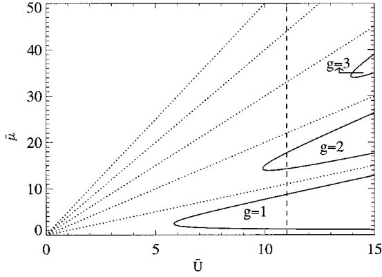
FIG. 2. Phase diagram of the Bose-Hubbard Hamiltonian as obtained from second-order perturbation theory (solid lines). The vertical axis shows the dimensionless chemical potential \bar{\mu} = \mu/zt and the horizontal axis shows the dimensionless interaction strength \bar{U} = U/zt . The dotted lines indicate the zeroth-order phase diagram. Later on, Fig. 5 is taken along the dashed line in this figure.
