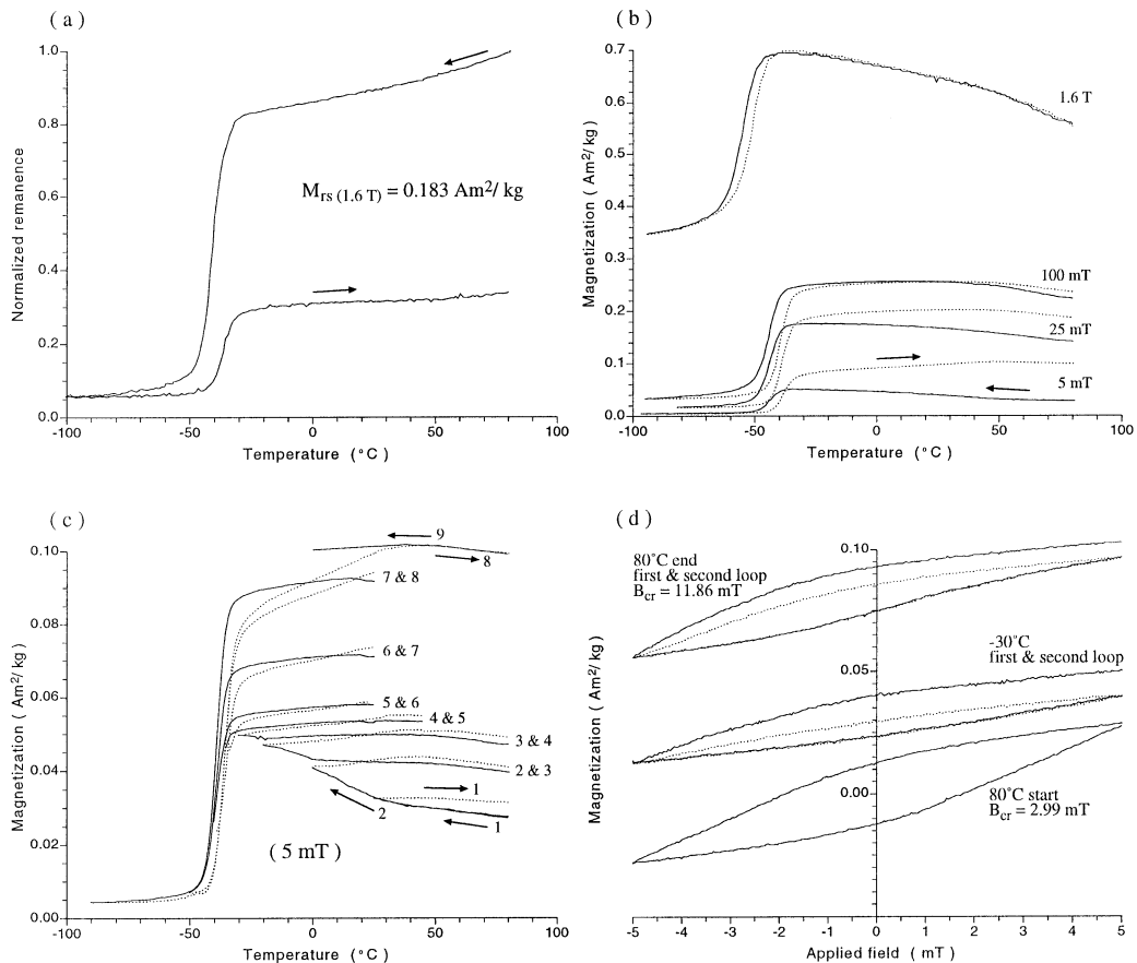
Figure 7. Various low-temperature MicroMag measurements obtained on LHC haematite (75–100 μm). (a) LT cycle of the saturation remanence (1.6 T). (b) LT cycles in various applied fields. (c) Repeated in-field cycling (5 mT) to increasingly lower temperatures. (d) Minor hysteresis loops (5 mT) obtained at different temperatures during an LT cycle through the Morin transition.
