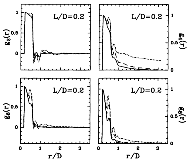
FIG. 9. Orientational distribution functions g_l(r) in the L/D = 0.2 system. For the definition of these functions, see Eq. (A1). The curves correspond to densities \rho^* = 0.51 (solid line), \rho^* = 0.57 (long-dashed line), and \rho^* = 0.63 (short-dashed line).
