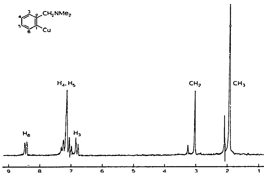
Fig. 3. 1 H NMR spectrum ( \delta ppm) of 2-[(dimethylamino)methyl]phenylcopper tetramer in benzene- d 6 .
