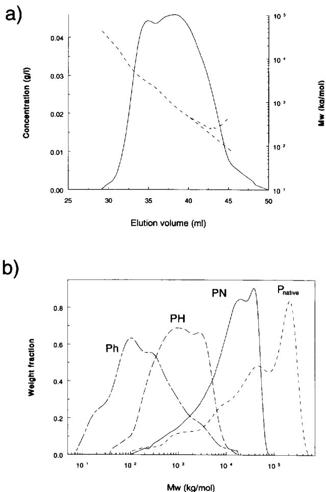
Figure 1 (a) Chromatogram (—) of the extruded PH TPS material with the calculated molecular masses (---). (b) Molecular mass distribution of the extruded Ph, PH and PN TPS materials in comparison with native potato starch ( P_{\text{native}} ), respectively from left to right
