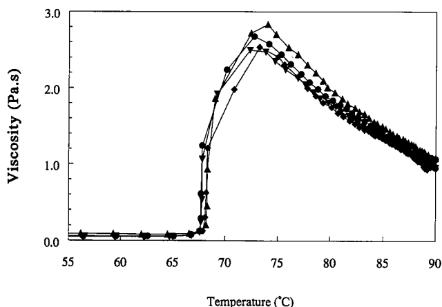
Figure 1 Viscograms of the four gels with 0% (◆), 1% (▼), 5% (●) and 20% (▲) glycerol
