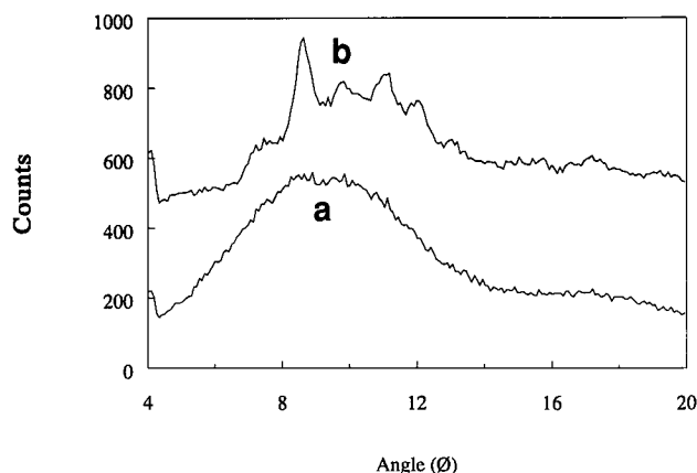
Figure 4 X-ray diffractograms of waxy maize after (a) 5 h and (b) 3 weeks of retrogradation
