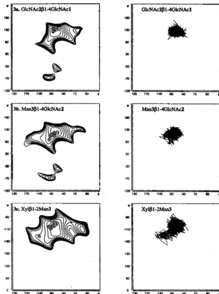
Fig. 3. Left column: HSEA energy contour plots of the disaccharide elements in the glycopeptide. Iso-energy contours are plotted at intervals of 1.5 kcal/mol with respect to the observed global energy minimum. Circles in the plots are positioned on the dihedral angle averages of the long MD trajectories A, B, C and of the conformational probes D1–D10. Within these circles, the signs +, – or \pm , respectively, indicate that the calculated interresidual NOE intensities across the glycosidic linkage are too large, too small or reasonably fit ( R_w < 25\% ) the experimental data. The signs of the glycosidic linkage of Man \alpha 1-6Man are based on the Man-4' H-1, Man-3 H-6 \text{proS} NOE intensities. Right column: combined \phi , \psi dihedral angles of all MD trajectories of the glycosidic linkages of the glycopeptide. Each picosecond of the total simulated time after equilibration (1560 ps) has been plotted. For the Man \alpha 1-6Man linkage, data are separated into gg ( \omega = -60 ) and gt ( \omega = 60 ) conformations.
