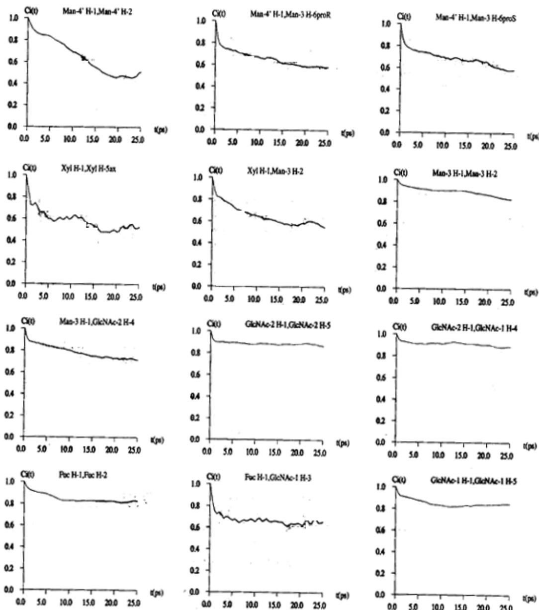
Fig. 4. Rotation correlation function plots of selected ^1\text{H} - ^1\text{H} pairs. The functions are calculated from the trajectory of run B from 20 to 70 ps, of which 25 ps are plotted.
