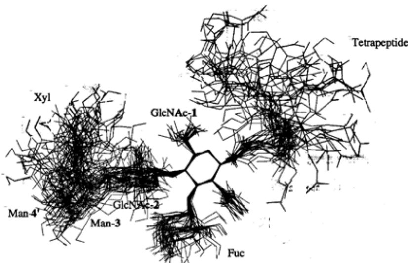
Fig. 2. Snapshots of structures of the glycopeptide, taken at intervals of 20 ps of the simulated trajectory of MD run A. The different conformations are superimposed on the GlcNAc-1 residue. Note that six gg and seven gt conformations for the Man \alpha 1-6Man linkage are present.
