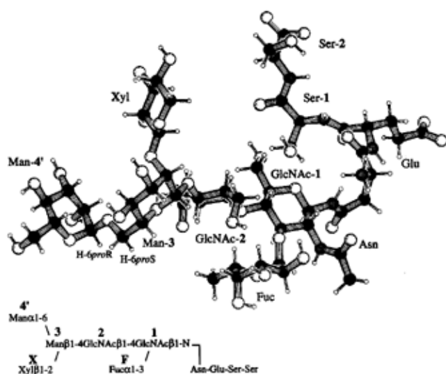
Fig. 1. The primary structure and a spatial model of the glycopeptide of pineapple stem bromelain.
