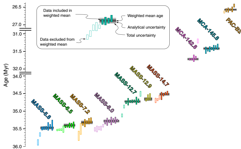
Figure 4. Plot of ranked ^{206}\text{Pb}/^{238}\text{U} dates from BRL from the Massignano, Monte Cagnero, and Pieve d'Accinelli sections. The total uncertainty of each weighted mean age includes the ^{238}\text{U} decay constant uncertainty and EARTHTIME U-Pb tracer calibration uncertainty. Note that the vertical time axis is not continuous.
