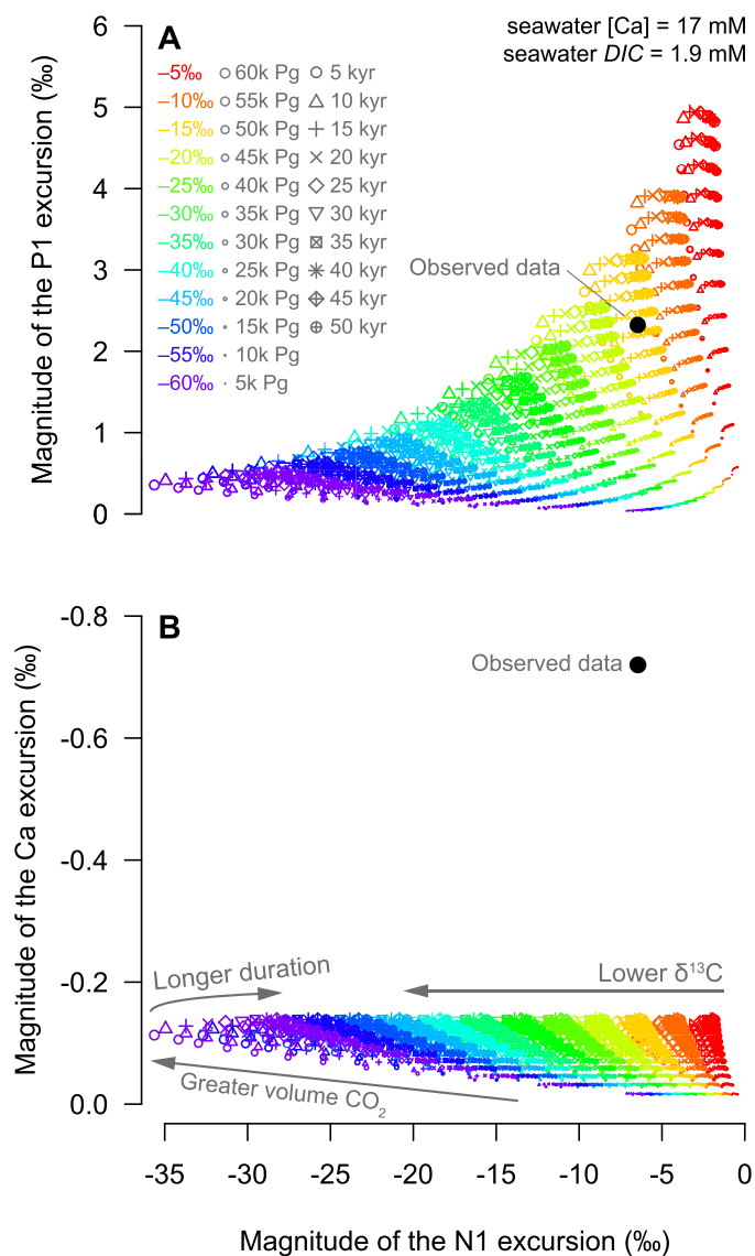
Figure 4. Model predicted (color) and observed (black) values for (a) the N1 and P1 \delta^{13}\text{C} excursions and (b) the N1 \delta^{13}\text{C} and \delta^{44/40}\text{Ca} excursion, demonstrating that while the \delta^{13}\text{C} data can be reconciled with modeled scenarios, the \delta^{44/40}\text{Ca} data cannot. For the model outputs, symbol size corresponds to the volume of injected \text{CO}_2 , symbol type corresponds to injection duration, and symbol color corresponds to the \delta^{13}\text{C} of the injected \text{CO}_2 . Model excursion magnitudes are relative to the preevent baseline. Observed \delta^{13}\text{C} excursion magnitudes are relative to the first sampled \delta^{13}\text{C} value at Val Adrara. The observed \delta^{44/40}\text{Ca} excursion magnitude is relative to the last data point ( -0.45\text{‰} ) before the excursion. While there is a range of scenarios that can replicate the \delta^{13}\text{C} data, there are no models that can simultaneously replicate the \delta^{44/40}\text{Ca} data.
