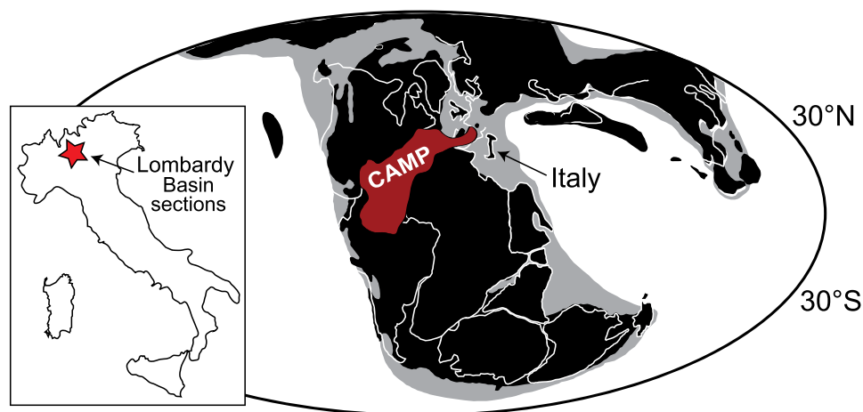
Figure 1. Paleogeographic reconstruction ~200 Ma showing the extent of CAMP and the location of Italy. Inset shows the location of the Lombardy Basin in Italy, where the Val Adrara (45°43'29.33"N, 9°57'32.29"E) and Italcementi (45°46'35.48"N, 9°30'27.09"E) sections are located. Modified from van de Schootbrugge et al. [2008] and Bachan et al. [2012].
