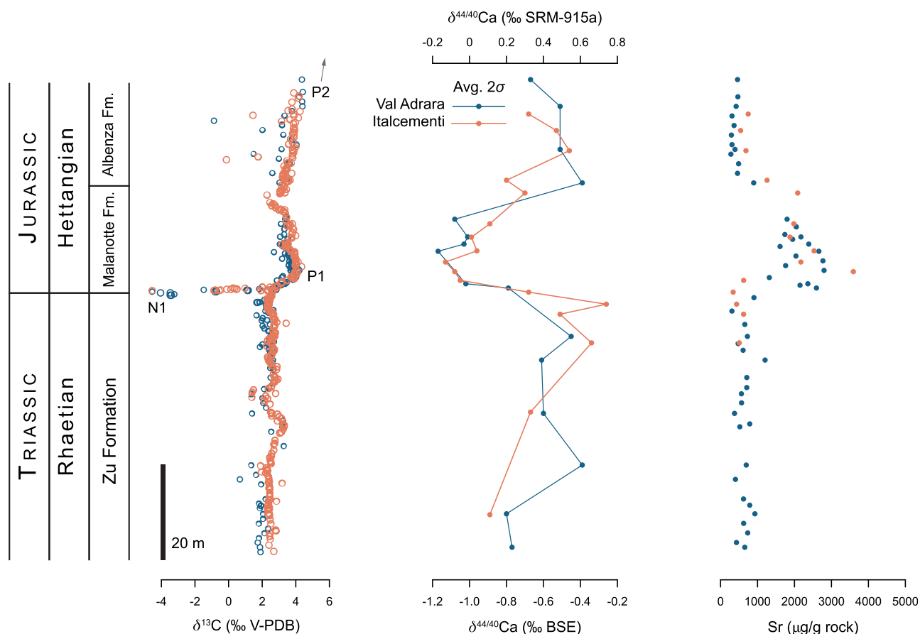
Figure 2. The \delta^{13}\text{C} , \delta^{44/40}\text{Ca} , and [\text{Sr}] data from each section, exhibiting large excursions immediately above the Triassic/Jurassic boundary. Dark blue is Val Adrara, orange is Italcementi. Val Adrara data are plotted by stratigraphic height, and Italcementi points are minimally adjusted to best match the \delta^{13}\text{C} patterns at Val Adrara. Errors on \delta^{44/40}\text{Ca} are calculated from replicate measurements of the same sample.
