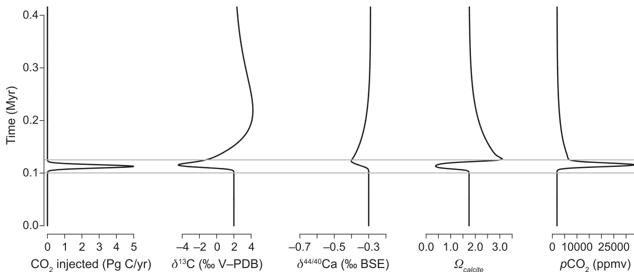
Figure 3. Output from a single model run illustrating the typical geochemical patterns resulting from a CO 2 perturbation in our model. From left to right, rate of CO 2 injection, \delta^{13}\text{C} , \delta^{44/40}\text{Ca} , \Omega_{\text{calcite}} , and p\text{CO}_2 . This scenario depicts an injection of 40,000 Pg C with a \delta^{13}\text{C} value of -15\text{‰} injected over 25 kyr. The grey lines signify the start and end of the CO 2 injection.
