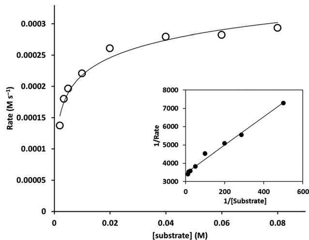
Fig. 7 A plot of the substrate concentration vs. the catalytic rate for [\text{Cu}_2^{\text{II}}(\text{L}^{\text{PzSSL}^{\text{Pz}}})(\text{Cl})_2](\text{BF}_4)_2 . The inset shows the Lineweaver–Burk plot. Reaction conditions: 0.4 mM [\text{Cu}] , 20 mM \text{NEt}_3 and varying amounts of 3,5-DTBC in 3 mL \text{CH}_3\text{CN} . V_{\text{max}} = 0.29 \text{ mM s}^{-1} ; K_{\text{m}} = 2.2 \text{ mM} ; k_{\text{cat}} = 5200 \text{ h}^{-1} .
