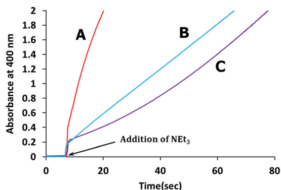
Fig. 6 Development in time of the absorption at 400 nm due to 3,5-DTBQ formation, catalyzed by [Cu II (L 1 SSL 1 )(Cl) 2 ](BF 4 ) 2 (red, type A), [Cu II (L 1 OH)(Cl)](BF 4 ) (blue, type B) and [Cu II (L Pz SSL Pz )(Cl) 2 ](BF 4 ) 2 (purple, type C).
