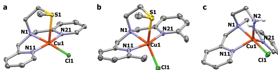
Fig. 5 Displacement ellipsoid plots (50% probability level) of the cationic parts of (a) [\text{Cu}^{\text{II}}(\text{L}^1\text{SCH}_3)(\text{Cl})](\text{BF}_4) , (b) [\text{Cu}^{\text{II}}(\text{L}^3\text{SCH}_3)(\text{Cl})](\text{BF}_4) and (c) [\text{Cu}^{\text{II}}(\text{L}^1\text{NH}_2)(\text{Cl})](\text{BF}_4) . The non-coordinating counterions and most of the hydrogen atoms are omitted for clarity.
