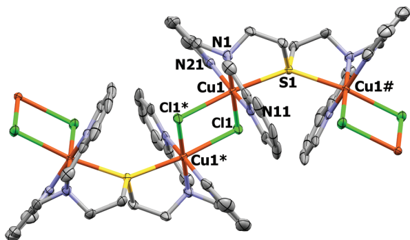
Fig. 3 Displacement ellipsoid plot (50% probability level) of two of the repeating units in the cationic polymer chain of [\text{Cu}_2^{\text{II}}(\text{L}^1\text{SL}^1)(\text{Cl})_2]_n(\text{BF}_4)_{2n} . The disorder, the non-coordinating counterions and hydrogen atoms are omitted for clarity. Symmetry operation * = [1 - x, -y, -z] and # = [1 - x, y, 1/2 - z] .
