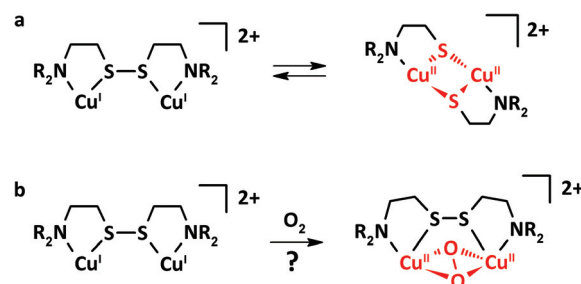
Fig. 1 Schematic representation of (a) the equilibrium between a Cu I disulfide and Cu II \mu -thiolate species and (b) the hypothesized reaction of a Cu I disulfide complex with O 2 to form a side-on Cu 2 II ( \mu - \eta^2 : \eta^2 -peroxide) species.
