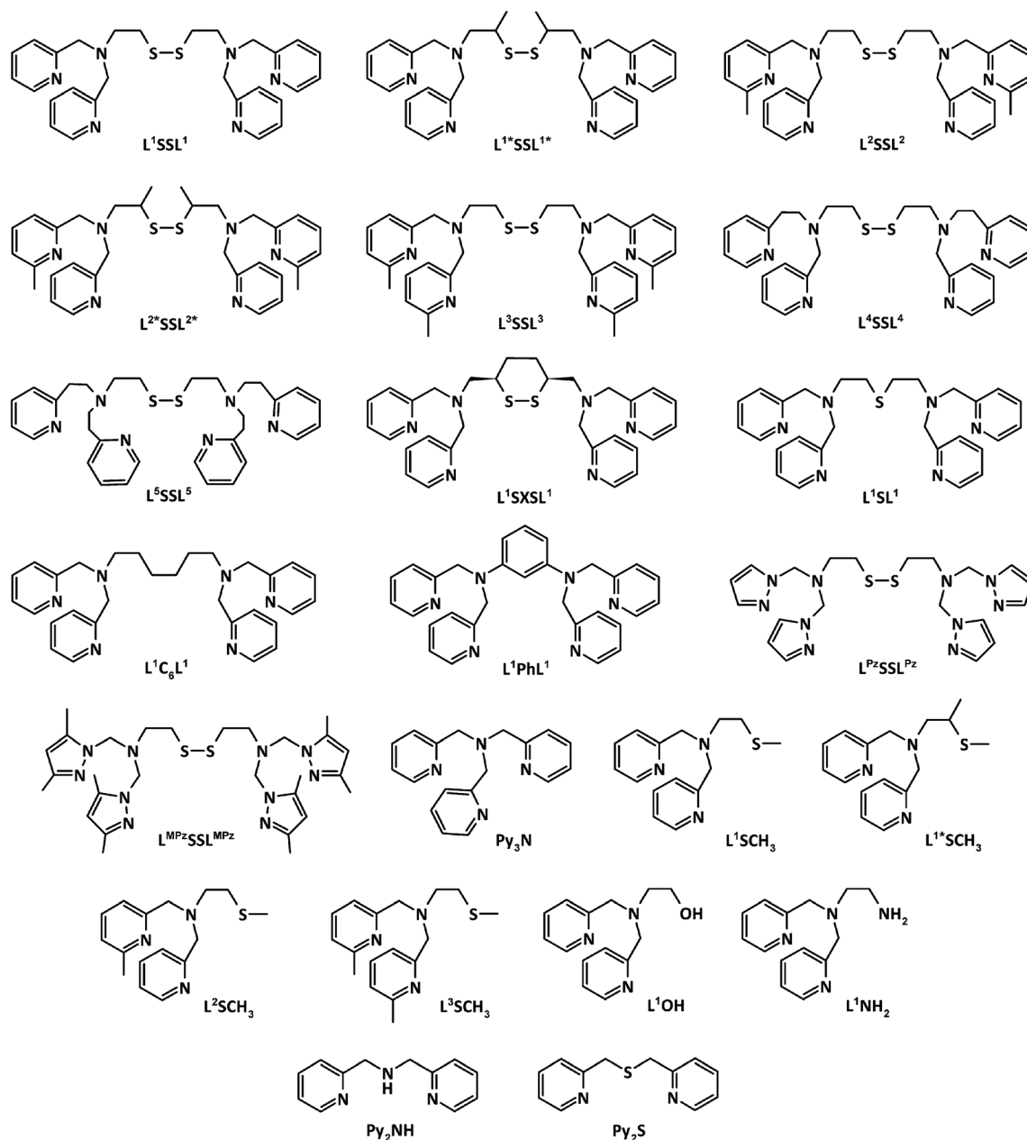
Fig. 2 Schematic overview of the ligands that were synthesized for the study of the copper-catalyzed oxidation of catechol.
