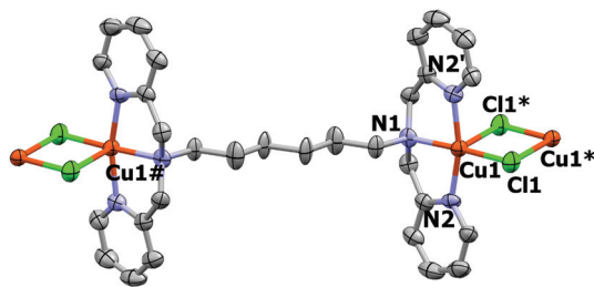
Fig. 4 Displacement ellipsoid plot (50% probability level) of the cationic part of [\text{Cu}^{\text{II}}(\text{L}^1\text{SCH}_3)(\text{Cl})]_2(\text{BF}_4)_{2n} . Non-coordinating \text{BF}_4^- counterions, acetonitrile solvent molecules and hydrogen atoms are omitted for clarity. Symmetry operation * = [1 - x, y, 1 - z] ; \# = [-x, y, -1 - z] ; ' = [x, -y, z] .
