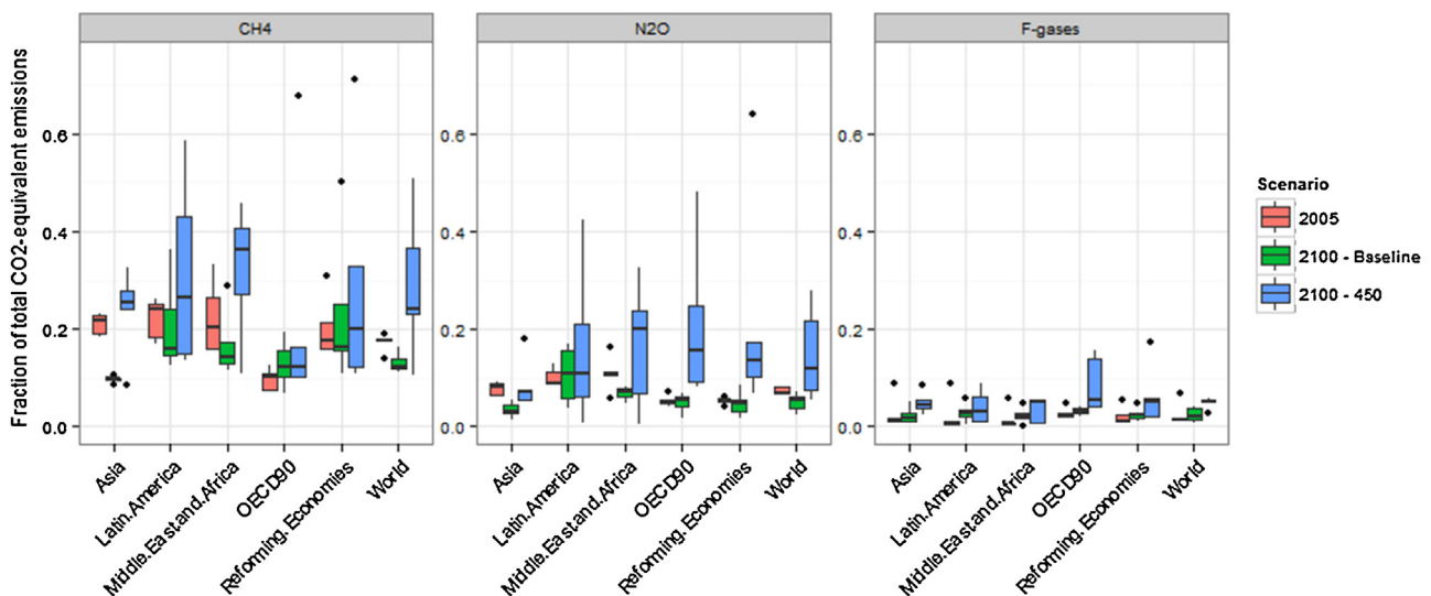
Fig. 11. Regional shares of non-CO 2 emissions. For the 450 scenario bio-CCS is excluded from the total regional emissions.
