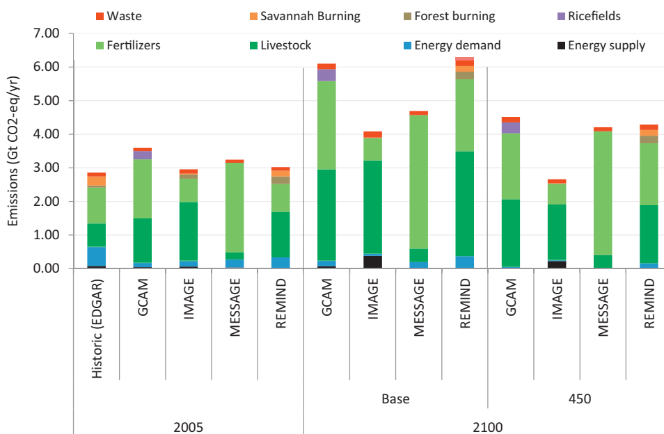
Fig. 7. Sectoral source N 2 O emissions in 2005 and 2100 in Baseline and 450 scenario. Note: Manure management emissions for the MESSAGE model are accounted for in the fertilizer sector.
