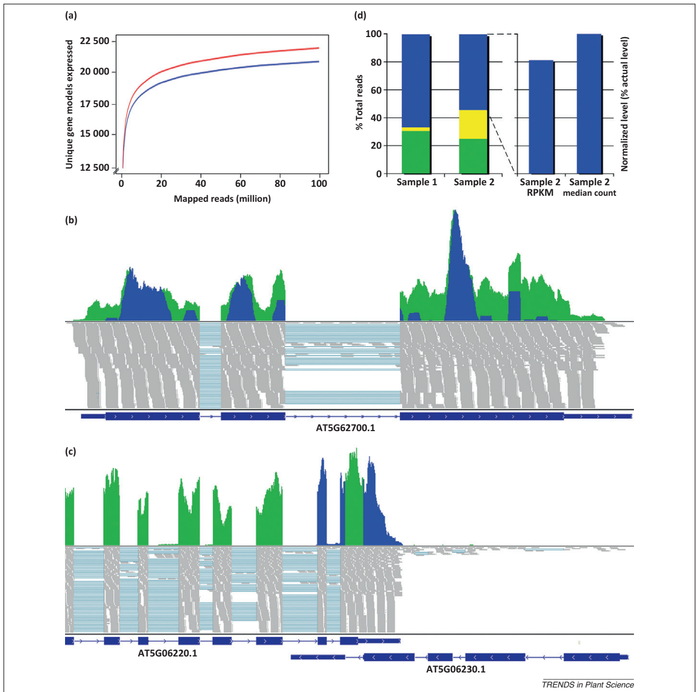
Figure 2. Considerations for next-generation RNA-seq data analysis. (a) Expression coverage versus total number of mapped reads. Reads (50 bp single end) from Arabidopsis leaf tissue were mapped to the genome. Read counts were summarized over annotated Arabidopsis gene models, with counts of four or more per gene defining expression when considering (red line) or omitting (blue line) multireads. Approximately 5% of aligned reads are multireads. In both scenarios, the number of genes that can be detected reaches a plateau at approximately 50 million reads. When multireads are considered 21 139 genes are detected. When multireads are omitted 20 162 genes are detected. In the latter case the 10th percentile gene has 19 reads. (b) Multireads can cause inaccurate expression estimates. Shown is read coverage for the TUBULIN BETA CHAIN 3 gene (AT5G62700). Gray lines indicate direct read alignments to the reference Arabidopsis genome and light blue lines indicate intron-spanning alignments of reads. The histograms show the combined contribution of unique reads and multireads that cover each base of this gene. Visualization was performed by the Integrative Genome Viewer (IGV) [18]. Per base coverage that originates from reads that uniquely map to this gene region are indicated in green, whereas in blue the per base coverage that is derived from alignments of reads that map to multiple regions in the genome (multireads) are indicated. In this example, inclusion of multireads would artificially inflate read coverage. (c) Overlap multireads can cause inaccurate expression estimates. Shown is read coverage for two genes that share a genomic region by overlap of their 3' ends on opposite strands. Reads that map to the region of overlap may originate from either transcript. In this example, the expression of the gene on the plus strand is markedly higher than of the gene on the minus strand, indicating that the vast majority of reads that align to the region of overlap originate from the gene on the plus strand. Random allocation of multireads would result in a severe overestimation of expression of the gene on the minus strand. (d) Normalization. The histogram in the left panel indicates the percentage of reads assigned to the 75 highest expressed genes (green + yellow) and to the remaining (relatively lower expressed) genes (blue) in two samples. There are no differences in read counts for every single gene in each sample except for only one of the highly expressed genes (yellow), which is 10-fold higher expressed in sample 2 compared with sample 1; this results in a higher contribution of the highly expressed genes to the total read count in sample 2. The choice of normalization method (explained in the main text) affects the analysis of differential expression levels between samples, as visualized in the histogram in the right panel. Normalized read counts for the individual genes in the relatively lower expressed gene set (blue) are correctly reflecting the actual counts when the median count normalization method is used. When using the RPKM normalization method, the normalized data are skewed due to the high expression difference of one gene (yellow), causing an underestimation of the expression level of all other genes of sample 2 to 80% of their actual expression levels, implying that all genes (in Arabidopsis over 30 000) would be falsely downregulated in sample 2 by 20% compared with sample 1. Abbreviation: RPKM, reads per kilobase of exon model per million mapped reads.
