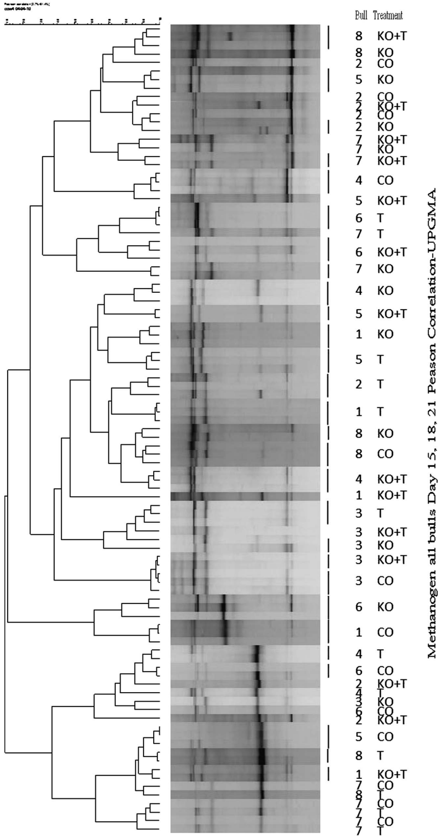
Figure 1 Cluster analysis of the denaturing gradient gel electrophoresis (DGGE) profile of Archaea present in the rumen of bulls on a total mixed ration supplemented (35 g/kg DM) with either beef tallow (T), coconut oil (CO), krabok oil (KO) or KO + T. To guarantee readability, the reference numbers of 'bull' and 'treatment' codes were combined when replicates clustered, as indicated by vertical lines next to the profile.
