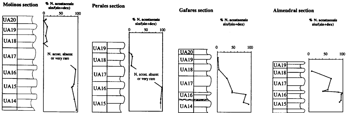
Fig. 6. Change in coiling direction from sinistral to dextral in the Neoglobobulid in the different sections.
